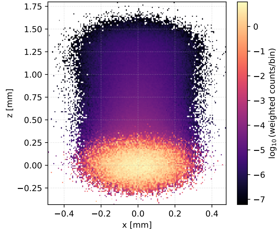
2D beam profile at sample (x focused only)
