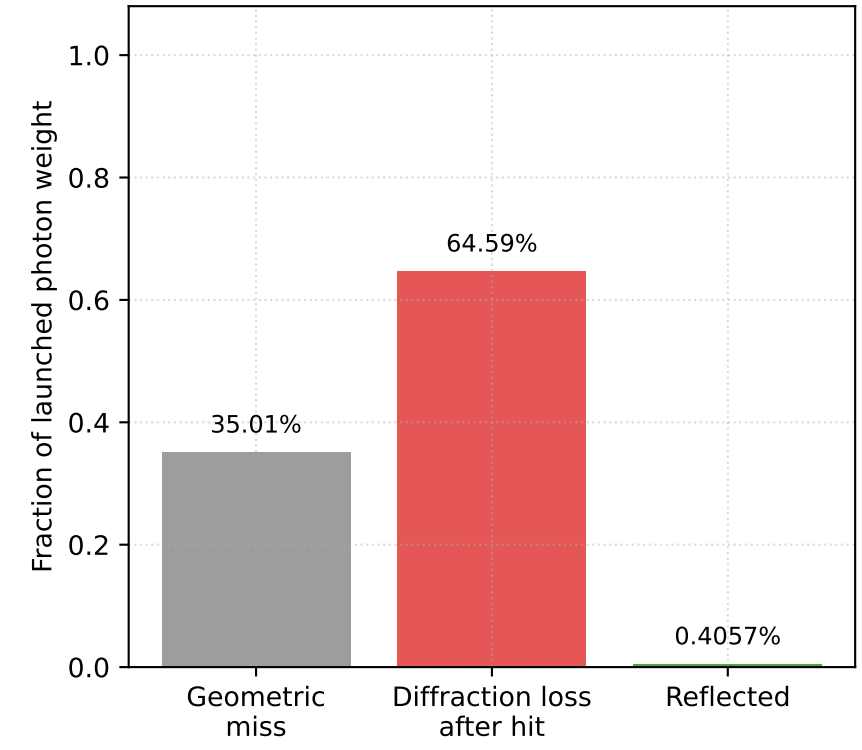
Exclusive throughput accounting
