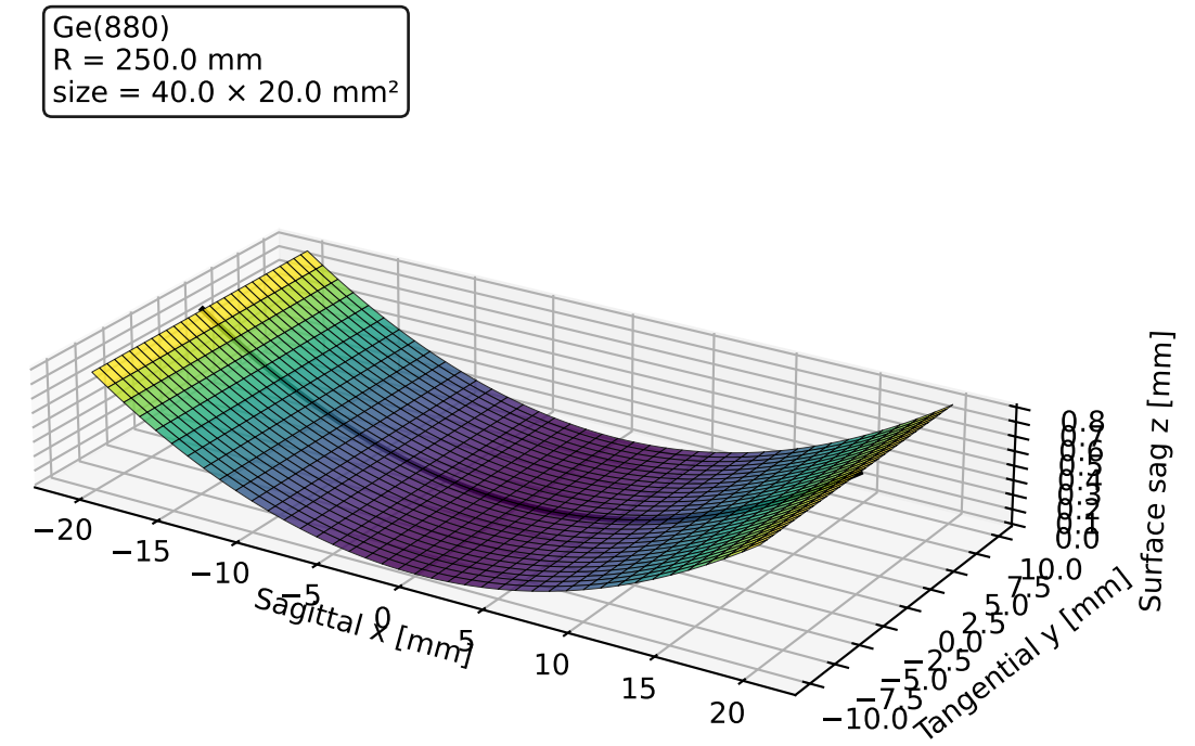
Sagittally curved crystal (local surface)
