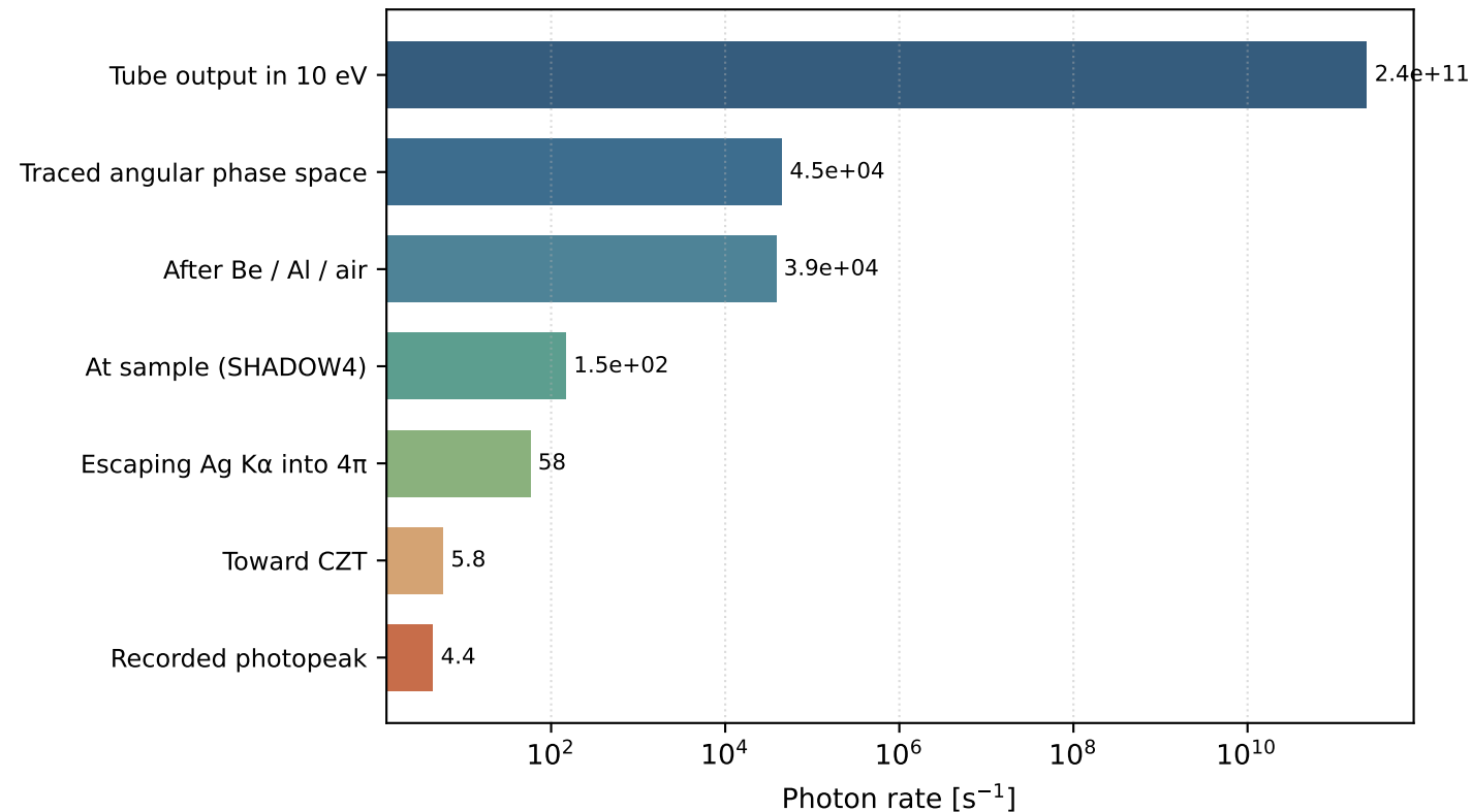
Ag K-edge photon-budget waterfall 40 kV, 2 kW W-tube screening case
