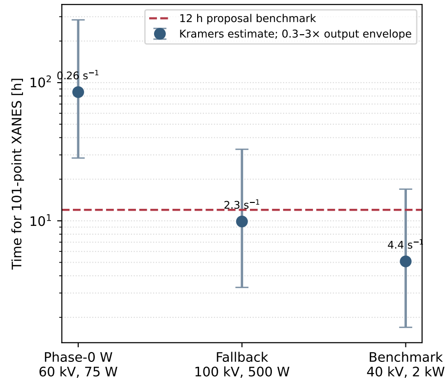
Conservative SNR=20 per point background/signal = 1
