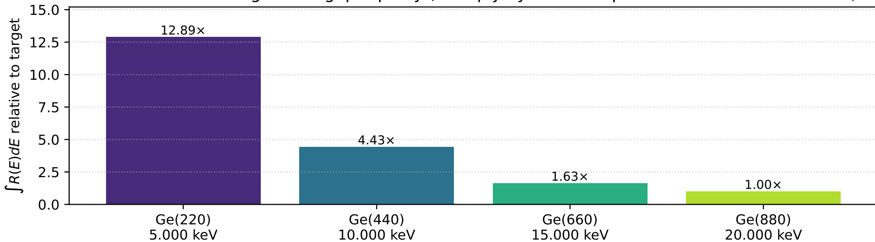
Broadband fixed-angle throughput proxy (multiply by incident spectral flux and transmission)
