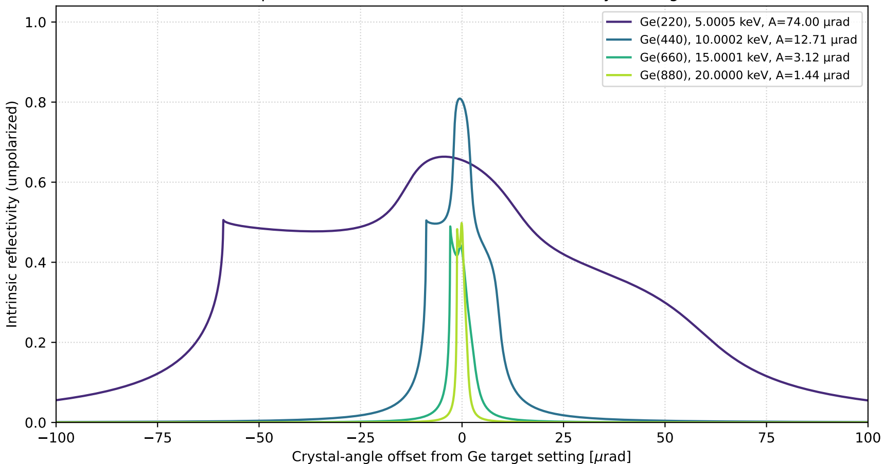
Lower orders parallel to Ge(880) at 20 keV; common crystal angle 38.3067°
