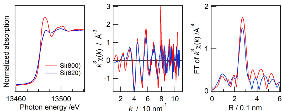
FIGURE 8 | Br K-edge XANES/EXAFS spectra of KBr with two types of monochromator crystals. Si(800): 80 s/pt. (XANES), 600 s/pt. (EXAFS); Si(620): 50 s/pt. (XANES), 180 s/pt. (EXAFS). [Colour figure can be viewed at wileyonlinelibrary.com ]
