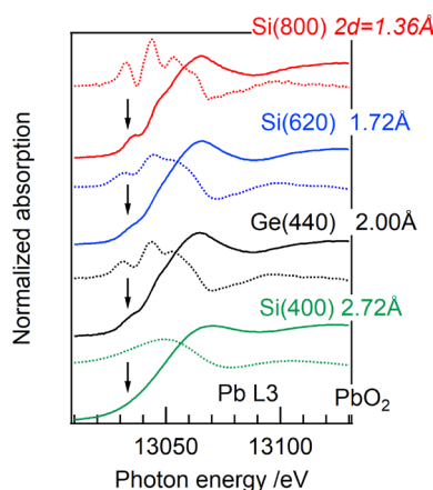
FIGURE 5 | Pb L3 edge XANES spectra of \text{PbO}_2 and the first derivatives recorded with four kinds of monochromator crystals. [Colour figure can be viewed at wileyonlinelibrary.com ]
