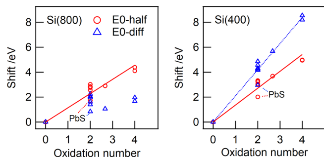
FIGURE 7 | Apparent absorption edge shift at the Pb L 3 edge from Pb metal, using different monochromator crystals and evaluation methods. E_0 -half: Energy at half of the normalized XANES. E_0 -diff: Energy at the peak of the first derivative spectrum. [Colour figure can be viewed at wileyonlinelibrary.com ]
