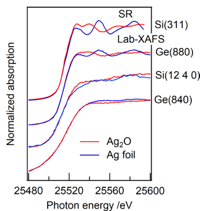
FIGURE 9 | Ag K-edge laboratory XANES spectra of Ag 2 O and Ag foil obtained using various monochromator crystals with different d-spacings. SR XANES was recorded at BL01B1 at SPring-8. [Colour figure can be viewed at wileyonlinelibrary.com ]
