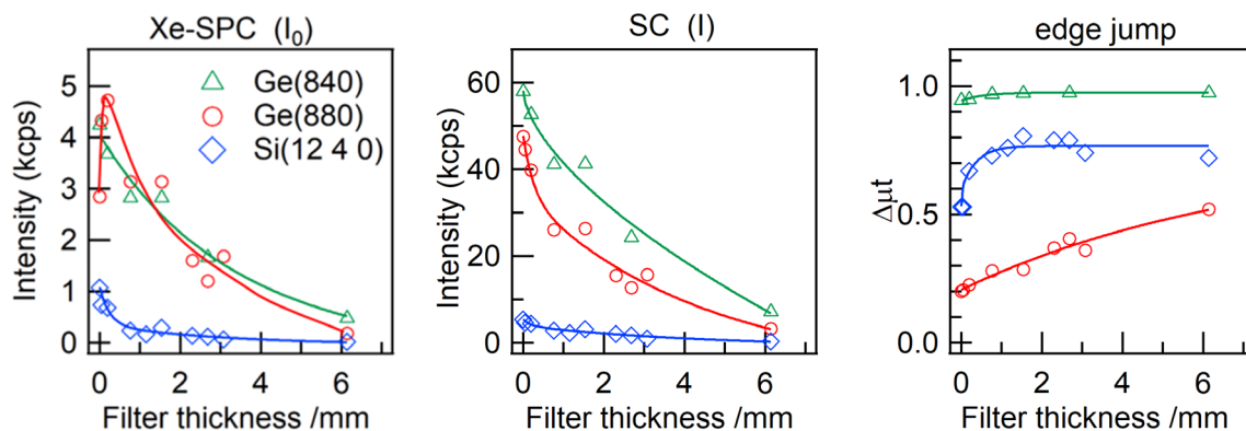
FIGURE 4 | Dependence of detected X-ray intensities at 25.4 keV on Al-filter thickness recorded with two different detectors and a monochromator crystal, and the resulting difference in the observed edge jump at Ag K-edge. Sample: 20 \mu\text{m} Ag foil. [Colour figure can be viewed at wileyonlinelibrary.com ]
