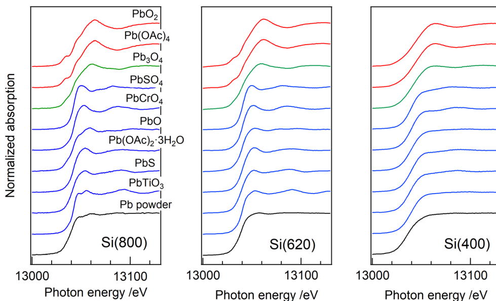
FIGURE 6 | Pb L3 edge XANES spectra of Pb compounds with different oxidation numbers and the coordination environment using three types of monochromator crystals. Conditions: Si(800): 21 kV, 50 mA, 150 s/pt., SS = 15 mm; Si(620): 27 kV, 50 mA, 100 s/pt., SS = 15 mm; Si(400): 27 kV, 20 mA, 30 s/pt., SS = 2 mm. [Colour figure can be viewed at wileyonlinelibrary.com ]
