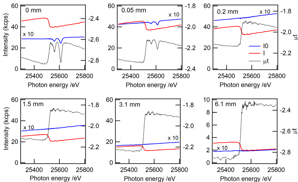
FIGURE 3 | Ag K-edge X-ray absorption spectra of Ag foil using various thicknesses of an Al filter. Monochromator crystal: Ge(880). Acquisition time: 50 s/pt. [Colour figure can be viewed at wileyonlinelibrary.com ]
