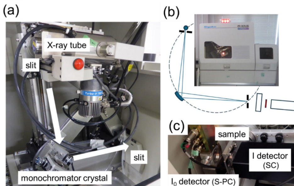
FIGURE 1 | The laboratory XAFS spectrometer and the schematic diagram. [Colour figure can be viewed at wileyonlinelibrary.com ]
