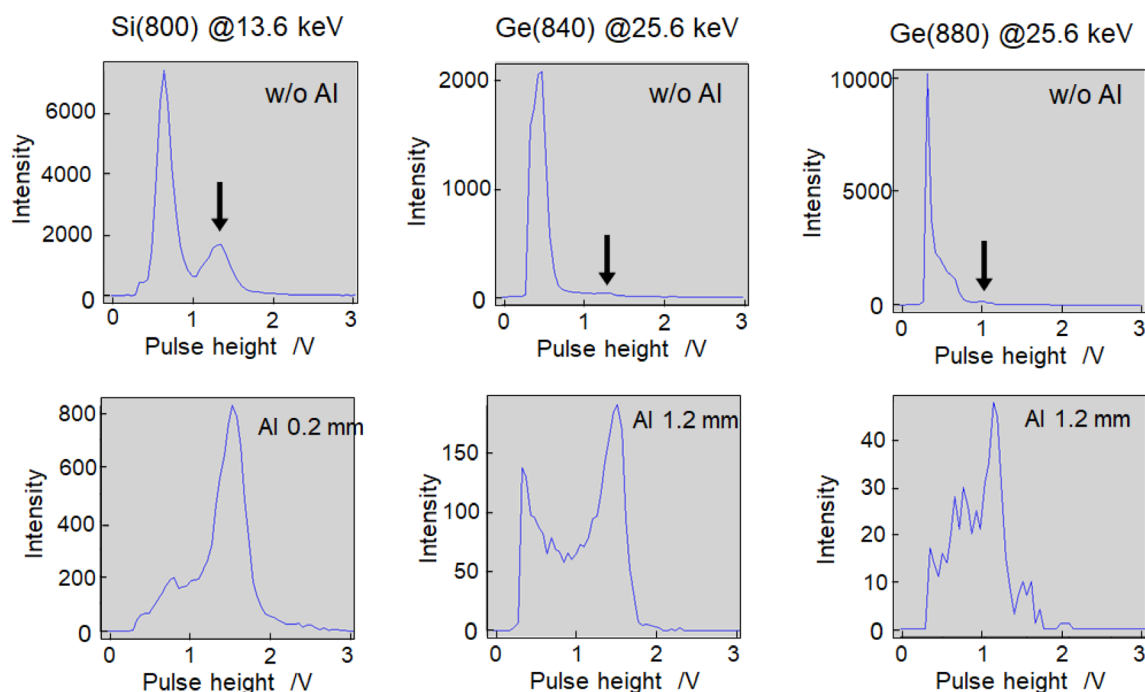
FIGURE 2 | Pulse height spectra of Xe-gas sealed proportional counter using Si(800), Ge(840) and Ge(880) monochromator crystal in the presence or absence of Al filter. Peaks indicated by arrows are due to X-rays of the target energy. [Colour figure can be viewed at wileyonlinelibrary.com ]
