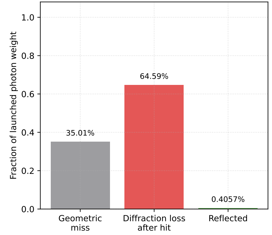
Exclusive throughput accounting
