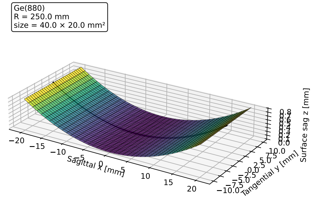
Sagittally curved crystal (local surface)
