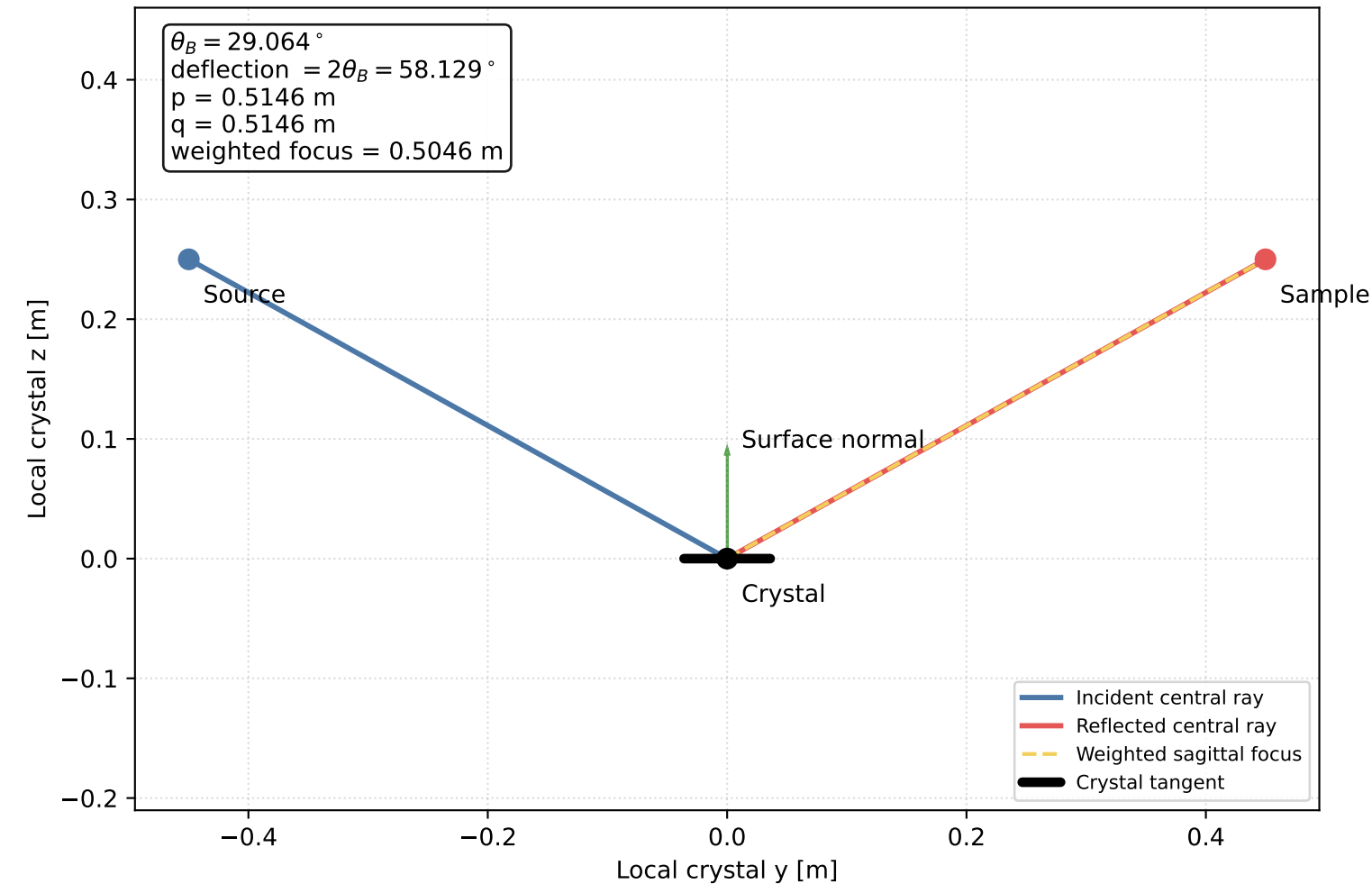
Central-ray layout in the diffraction plane
