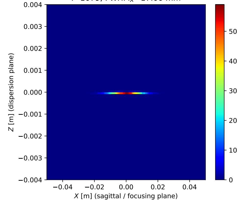
(a) image at q = 10 m, mosaicity 0.2^\circ FWHM l=1079 , \text{FWHM}_X=17.00 mm
