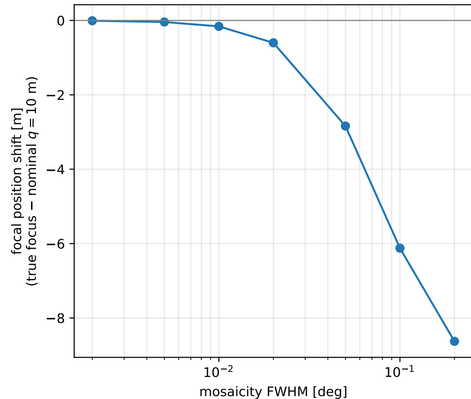
(c) focal position shift vs mosaicity (geometry, p = q = 10 m, fixed)
