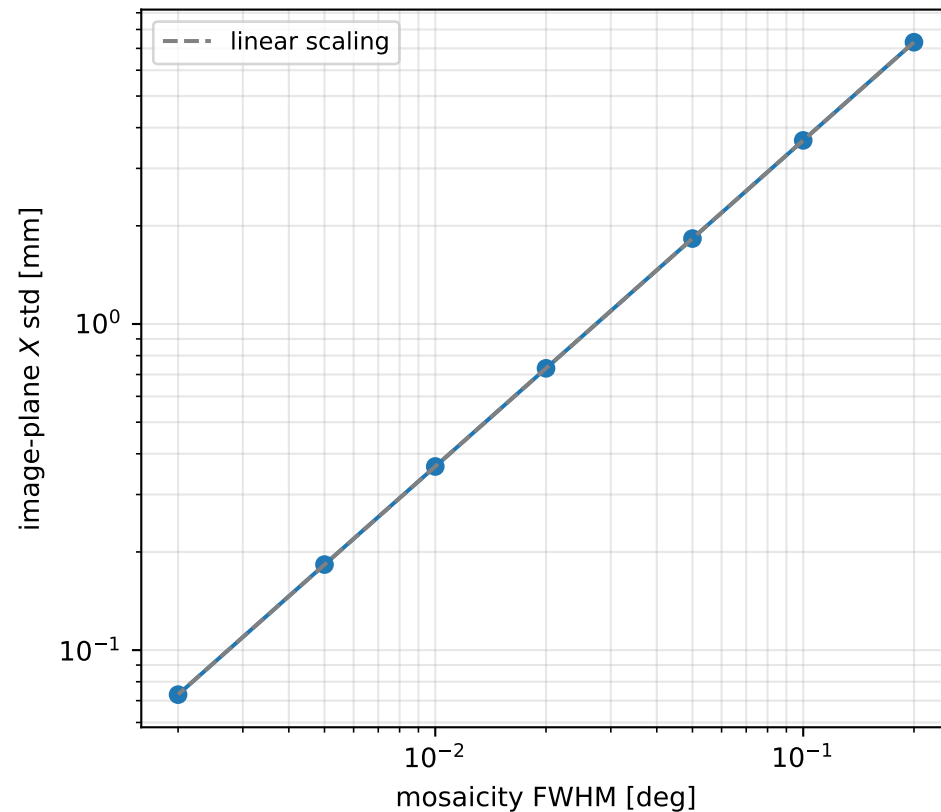
(b) image blur vs mosaicity (geometry, p = q = 10 m, fixed)
