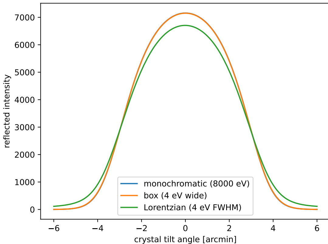
Rocking curves for different source spectra (mosaicity 0.05^\circ FWHM)
