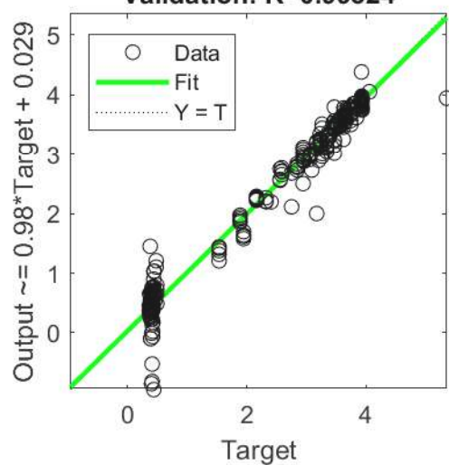
Validation: R=0.99324
