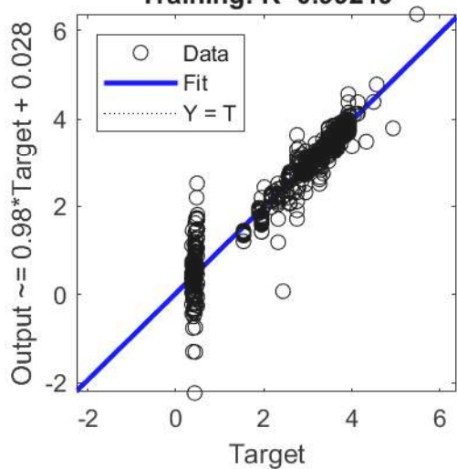
Training: R=0.99219
