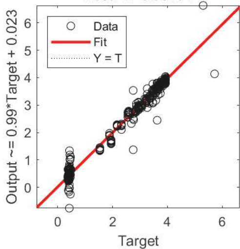
Test: R=0.99291
