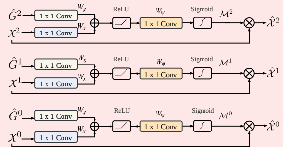
Student Network
