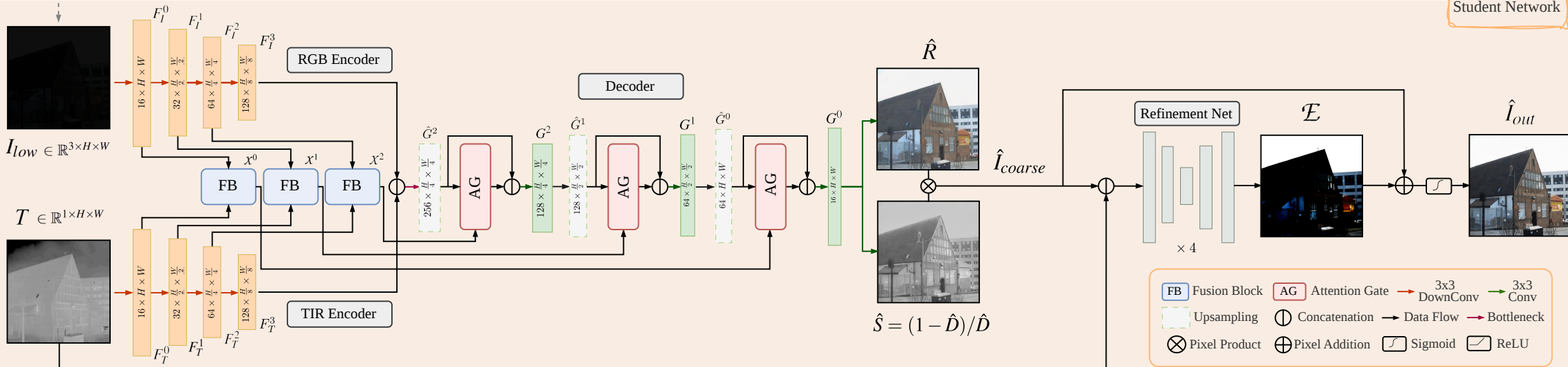
Student Network
