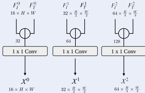
Fusion Block
