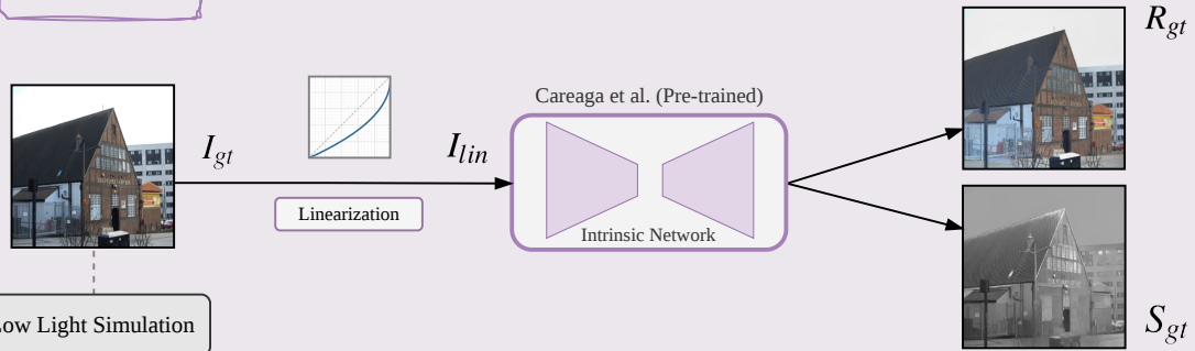
Teacher Network
