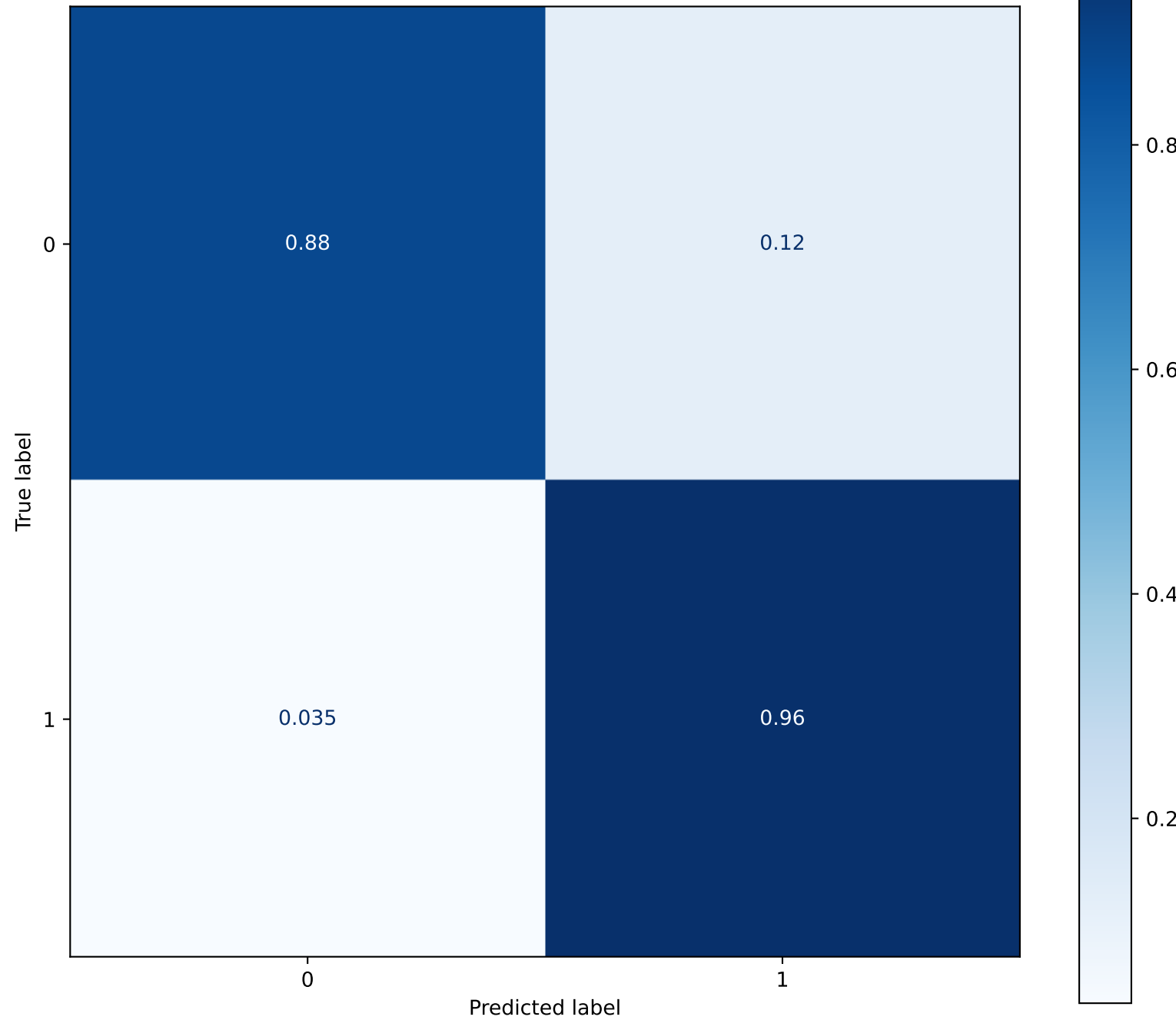
Confusion Matrix - Binary Classification (0: Normal, 1: Attack)
