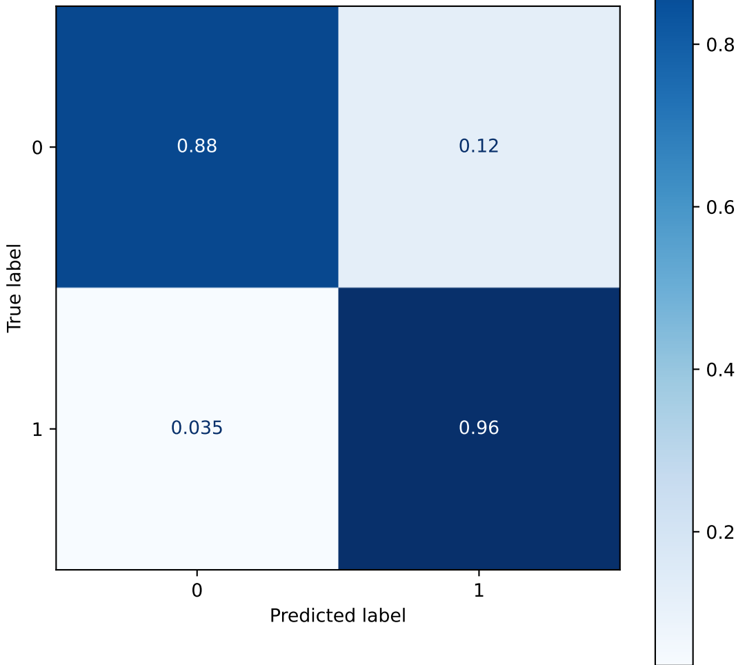
Confusion Matrix - Binary Classification (0: Normal, 1: Attack)
