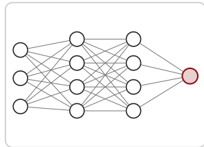
Neural networks
