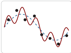
Overfitting
