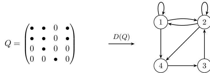
Figure 1: A 4 \times 4 upper Hessenberg matrix ( \bullet = \text{nonzero} ) and its support digraph D(Q) . Each nonzero entry Q_{ij} becomes a directed arc i \rightarrow j .
