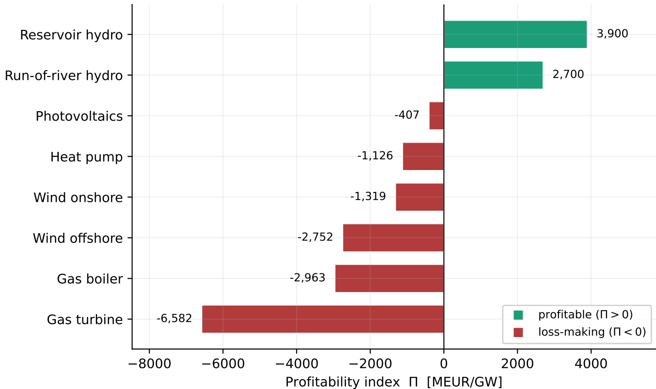
Clean year-0 profitability index per technology ( \omega -invariant)
