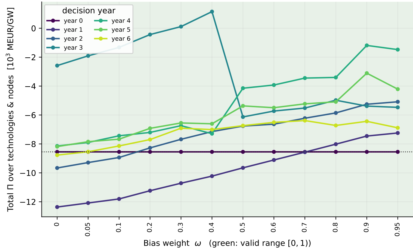
Endogeneity of \Pi : \Pi drifts upward with \omega (years \geq 1 )
