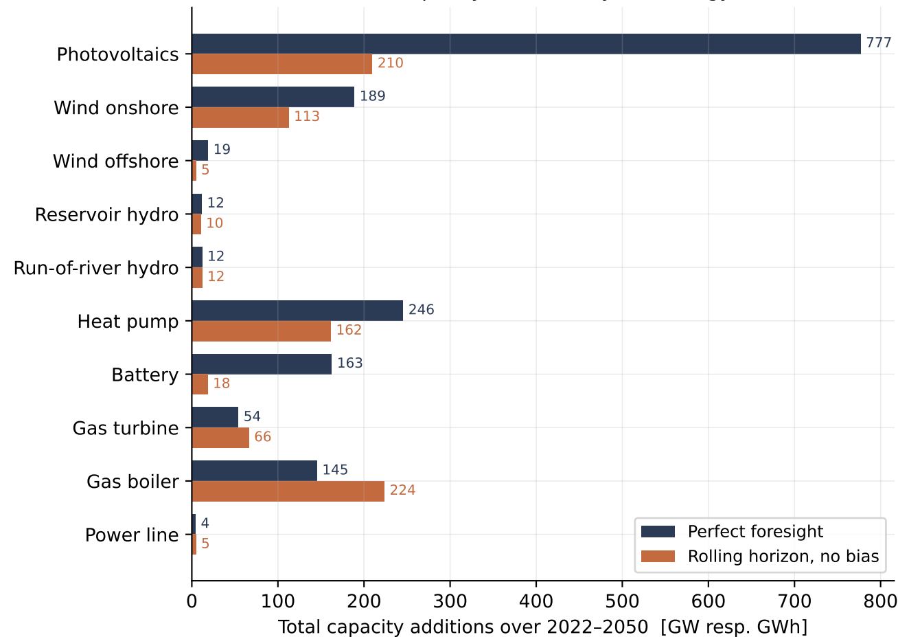
(a) Capacity additions by technology
