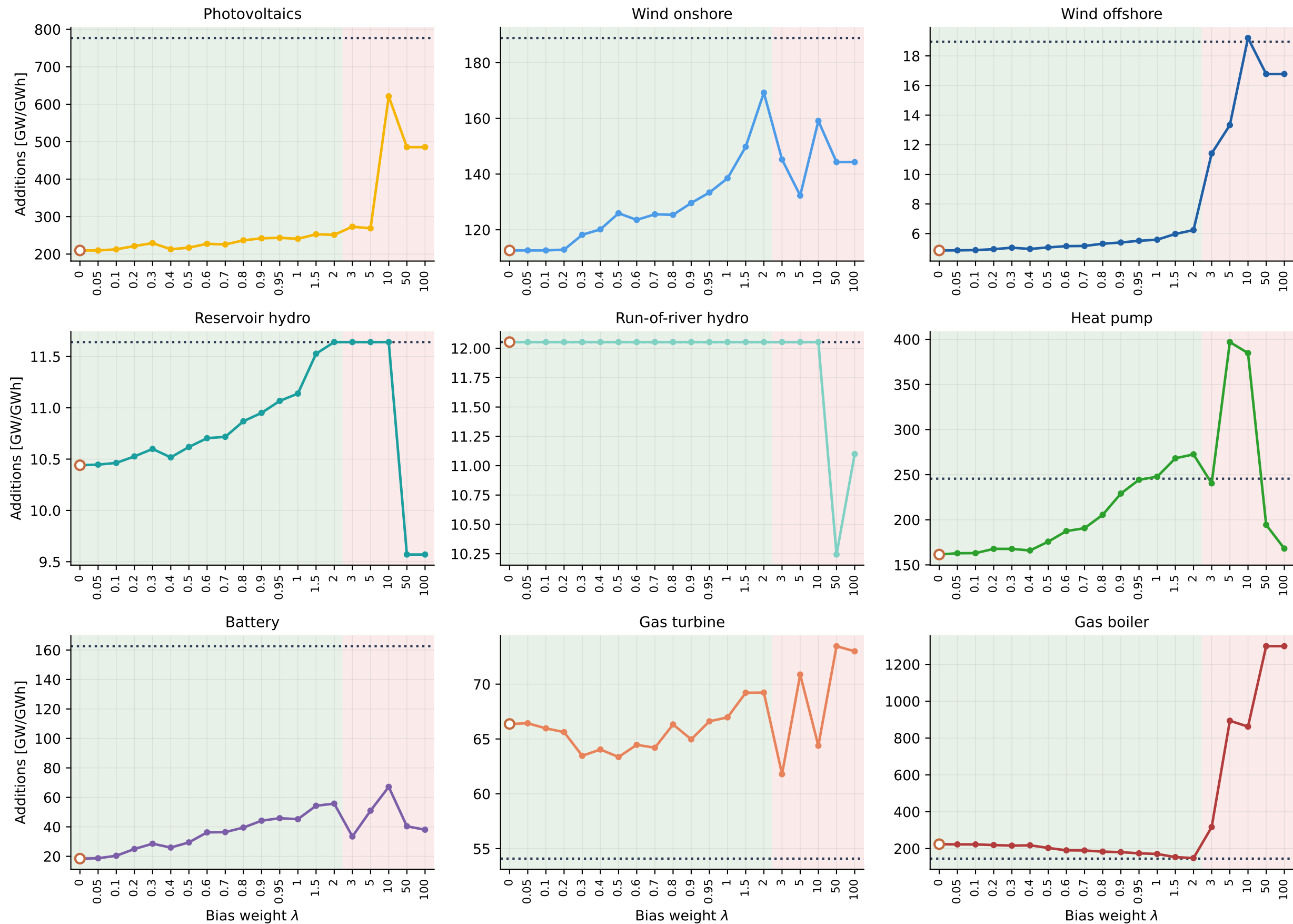
Capacity additions per technology vs. bias weight (rolling horizon, no policy)
