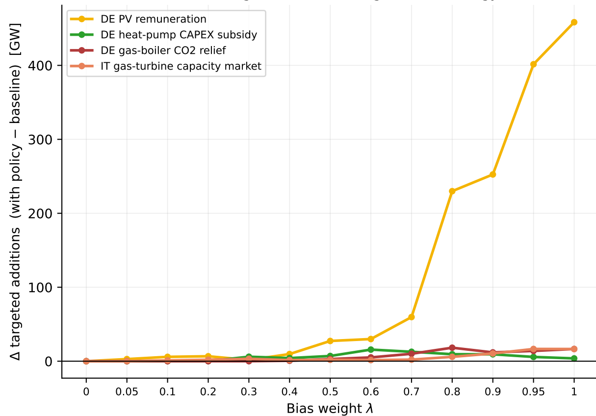
(a) Steering effect on the targeted technology
