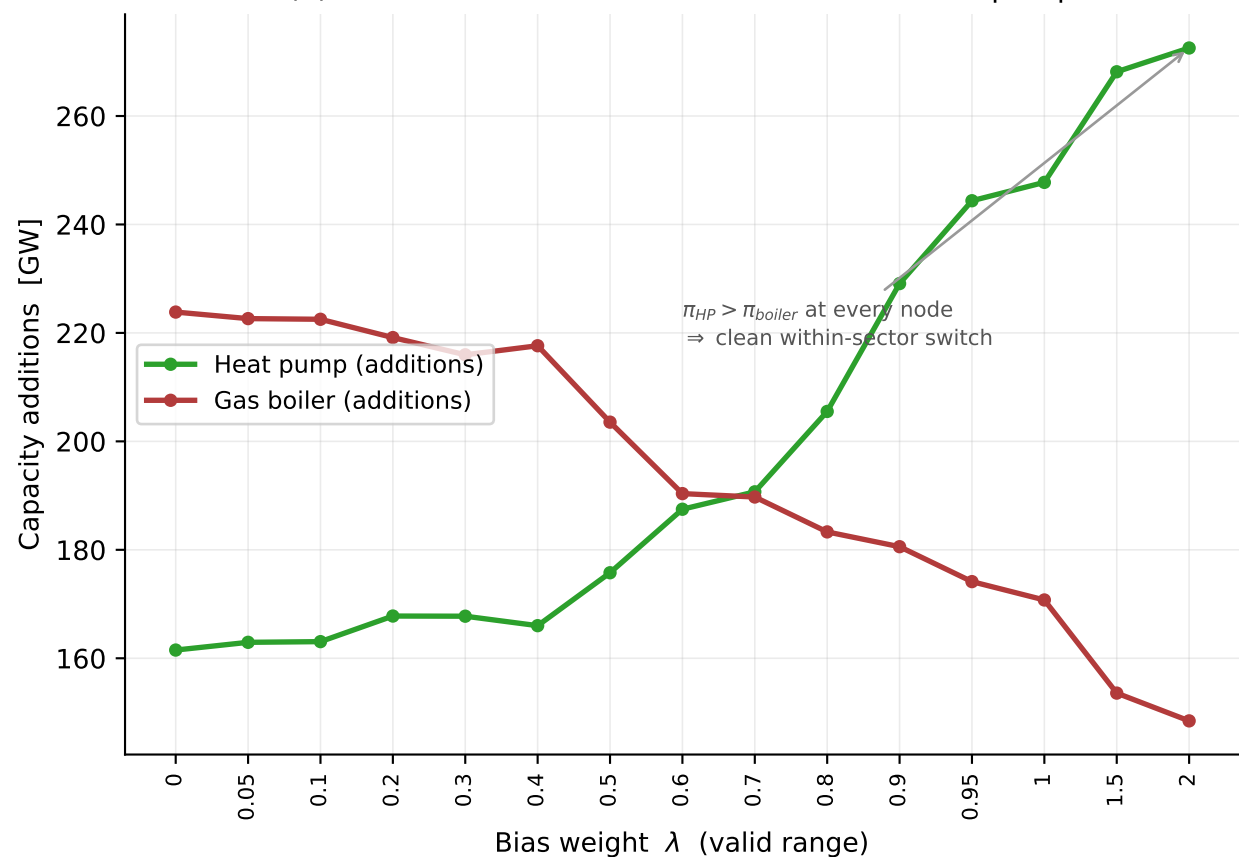
(b) Heat sector: bias substitutes boiler \rightarrow heat pump
