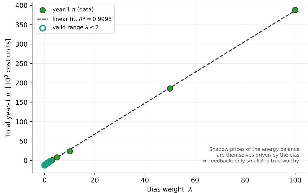
(b) Year-1 \pi scales linearly with \lambda
