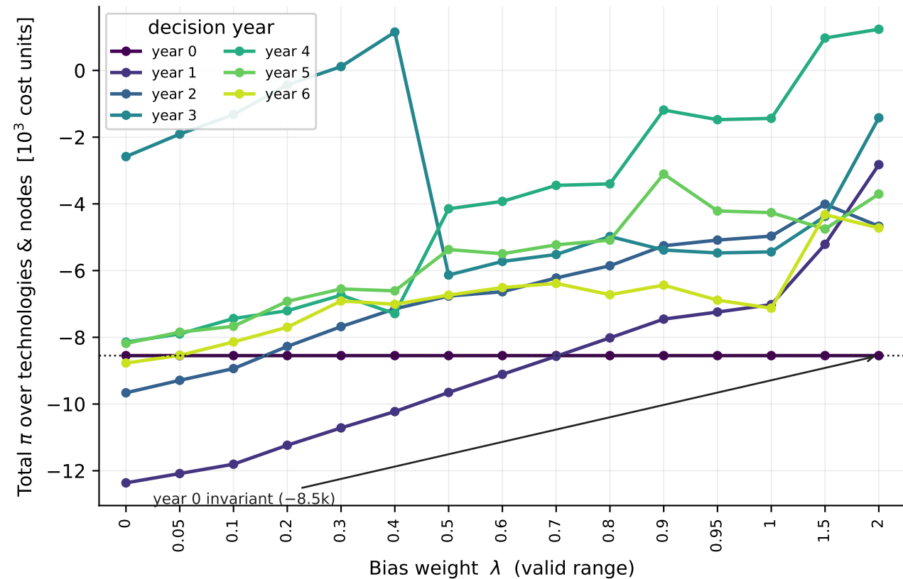
(a) \pi drifts upward with \lambda (years \geq 1 )
