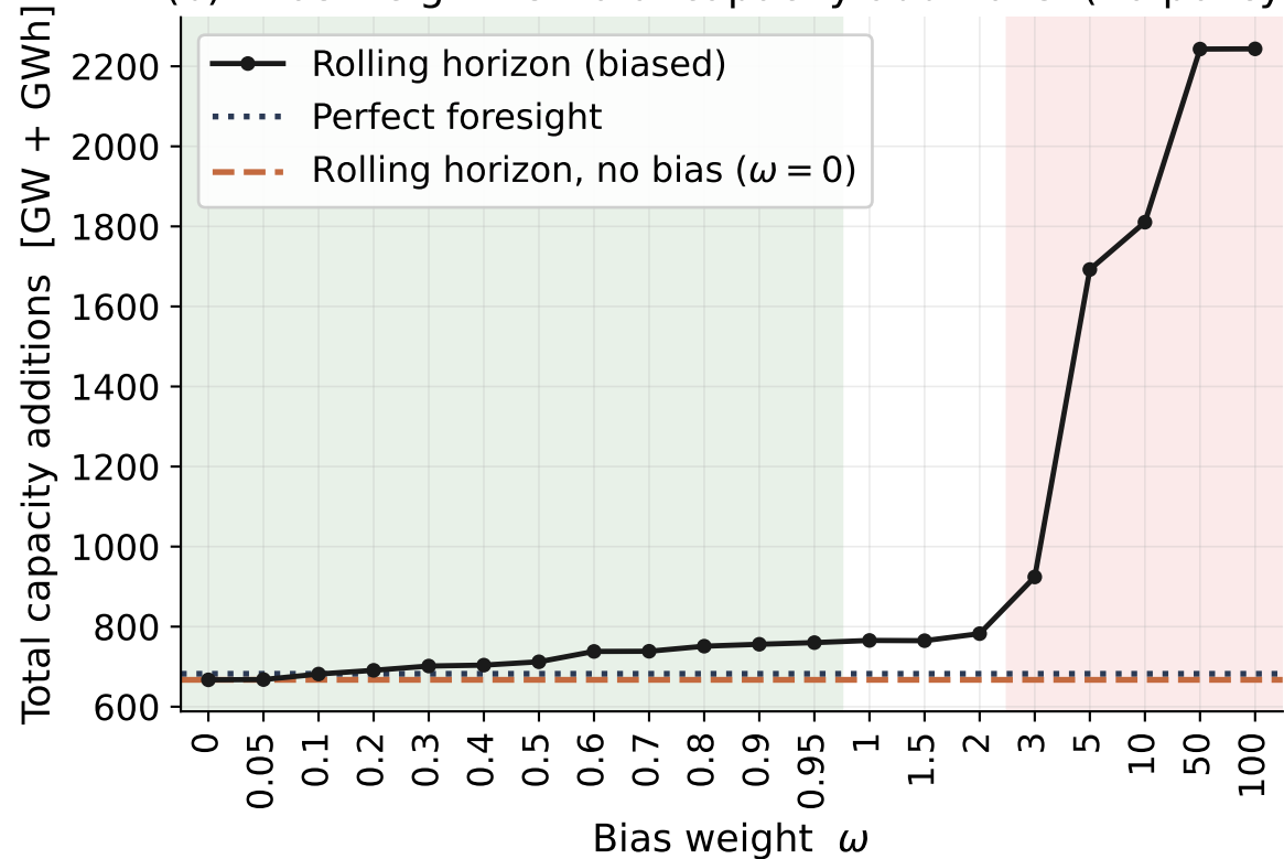
(b) Bias weight vs. total capacity additions (no policy)
