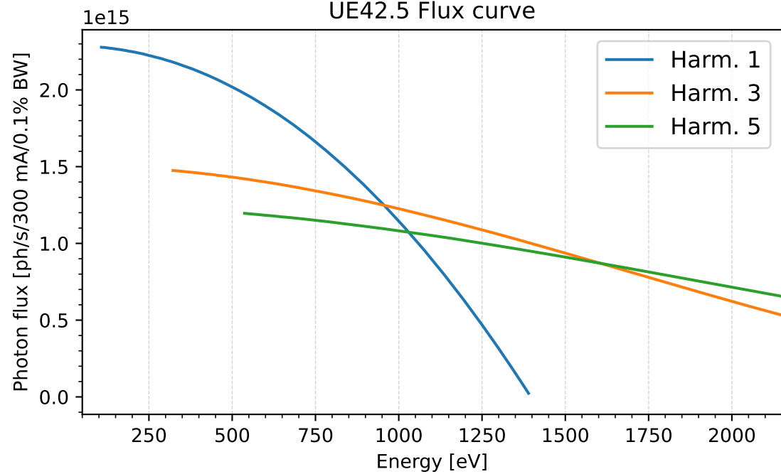
Transmitted flux (Flux on sample)
