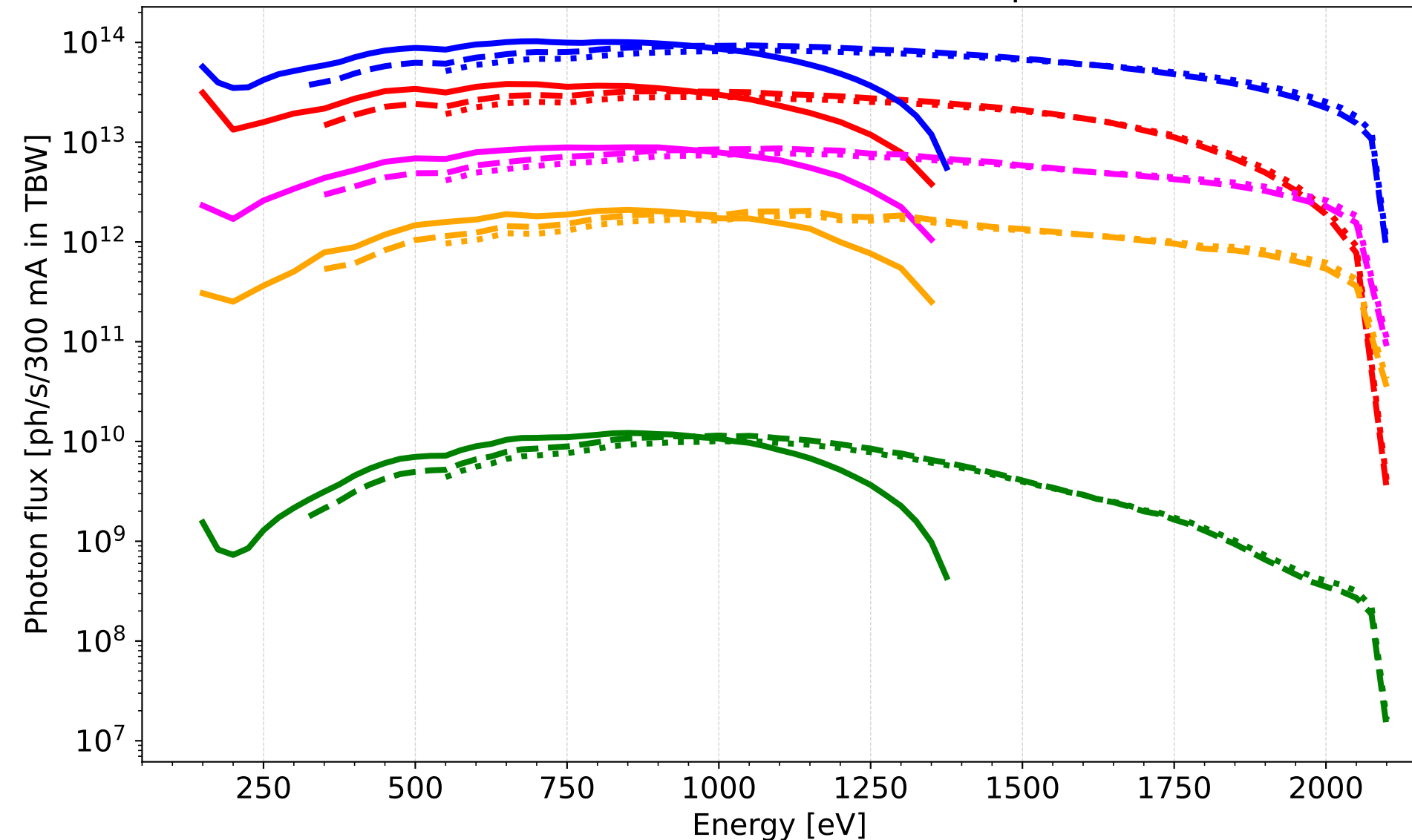
Transmitted flux (Flux on sample)
