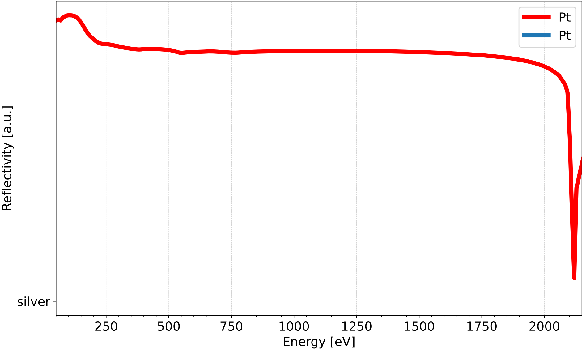
Mirror Coating Reflectivity @ 0.75° incident angle
