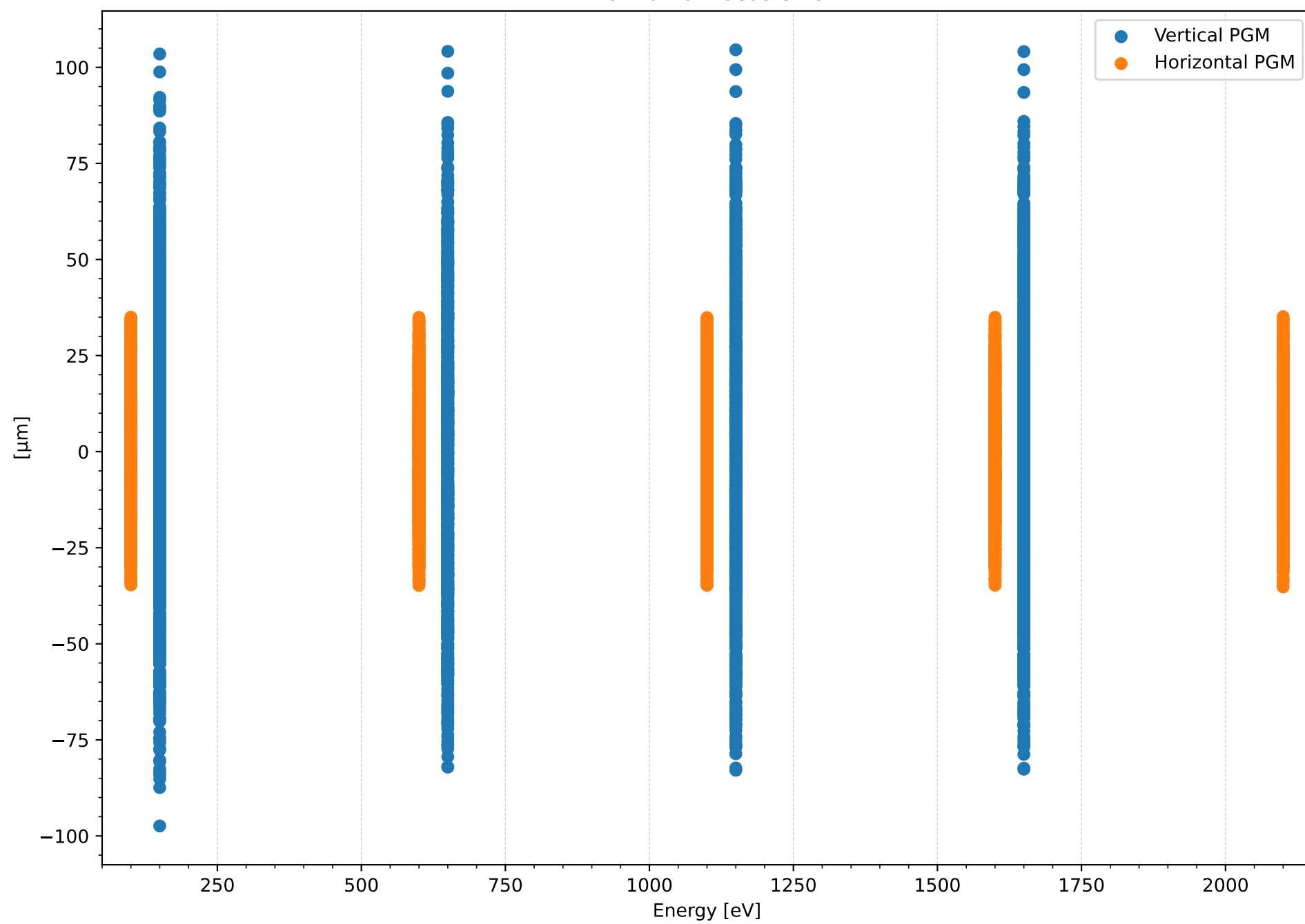
Horizontal Focus Size
