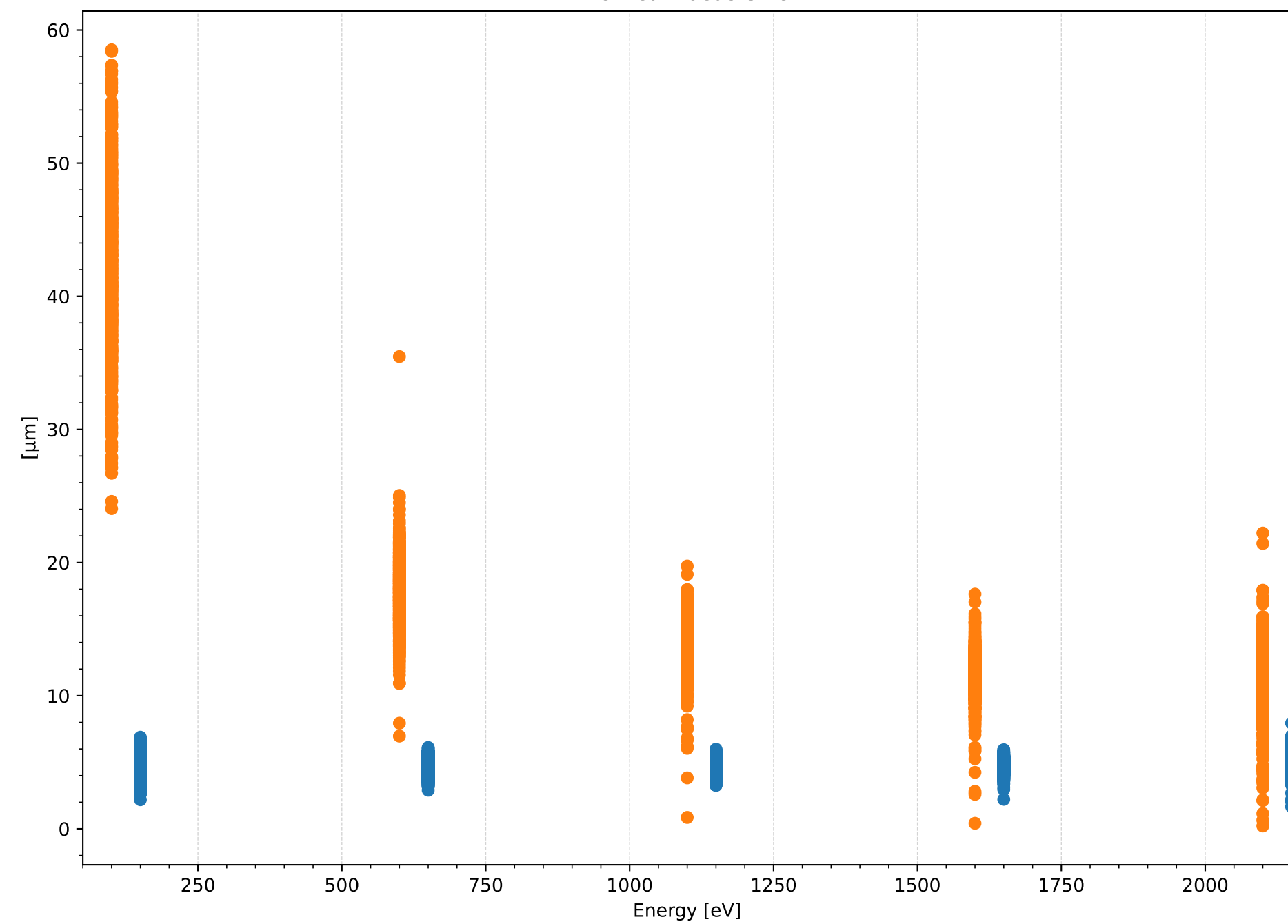
Vertical Focus Size
