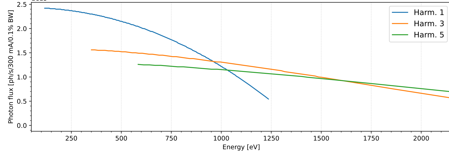
Transmitted flux 100 m HR-RIXS Beamline
