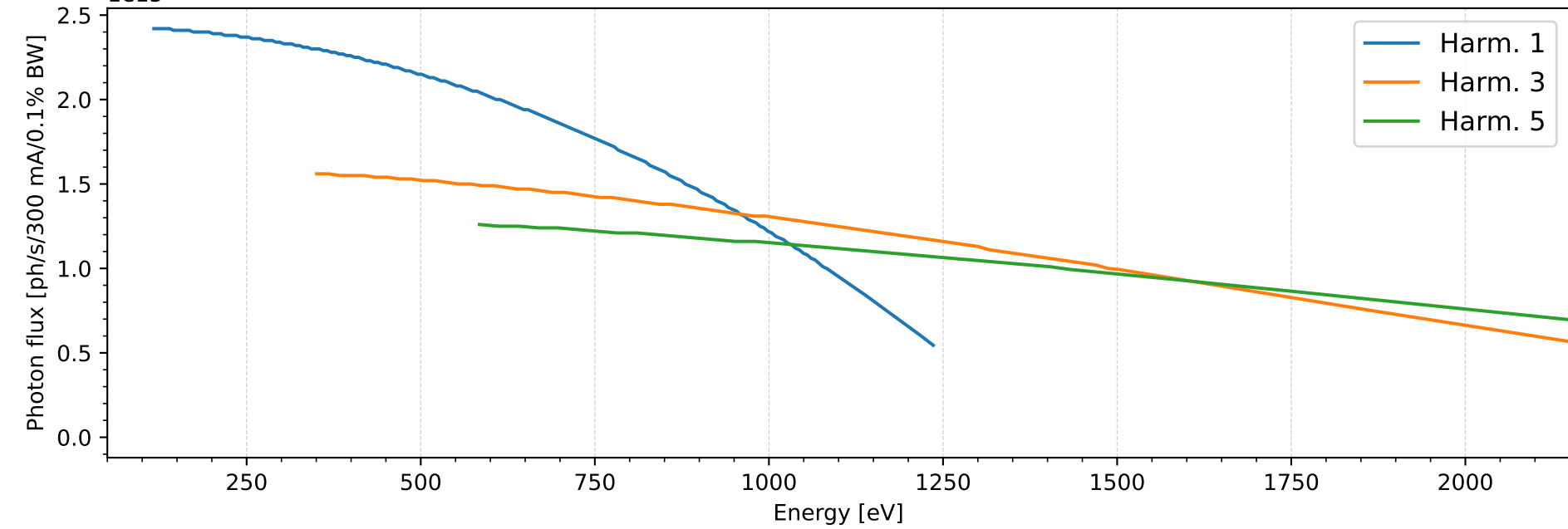
Transmitted flux 91 m HR-RIXS Beamline
