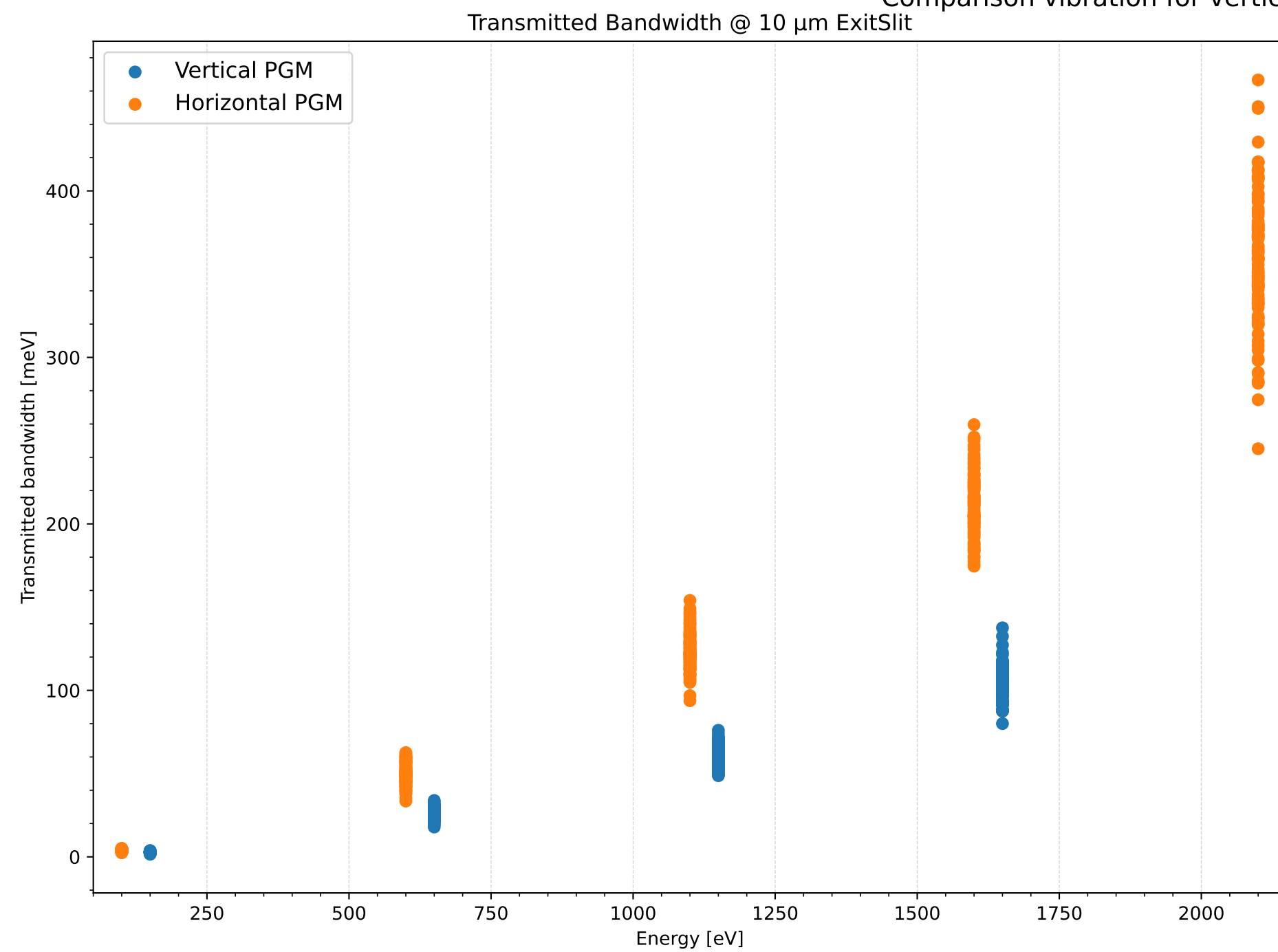
Comparison vibration for vertical/horizontal PGM, amplitude: 0.0003
