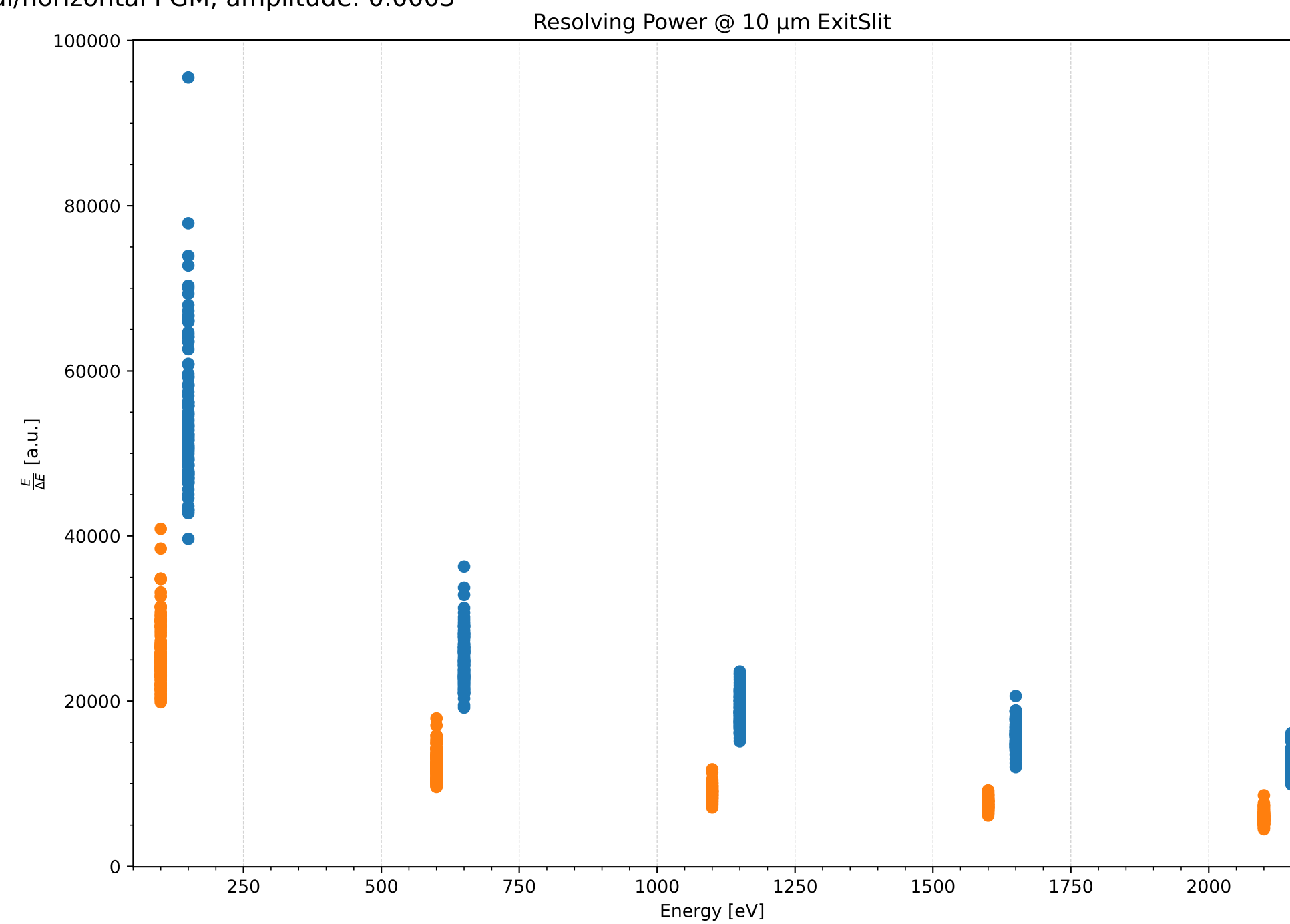
Comparison vibration for vertical/horizontal PGM, amplitude: 0.0003
