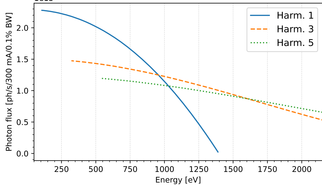
Transmitted flux (Flux on sample)
