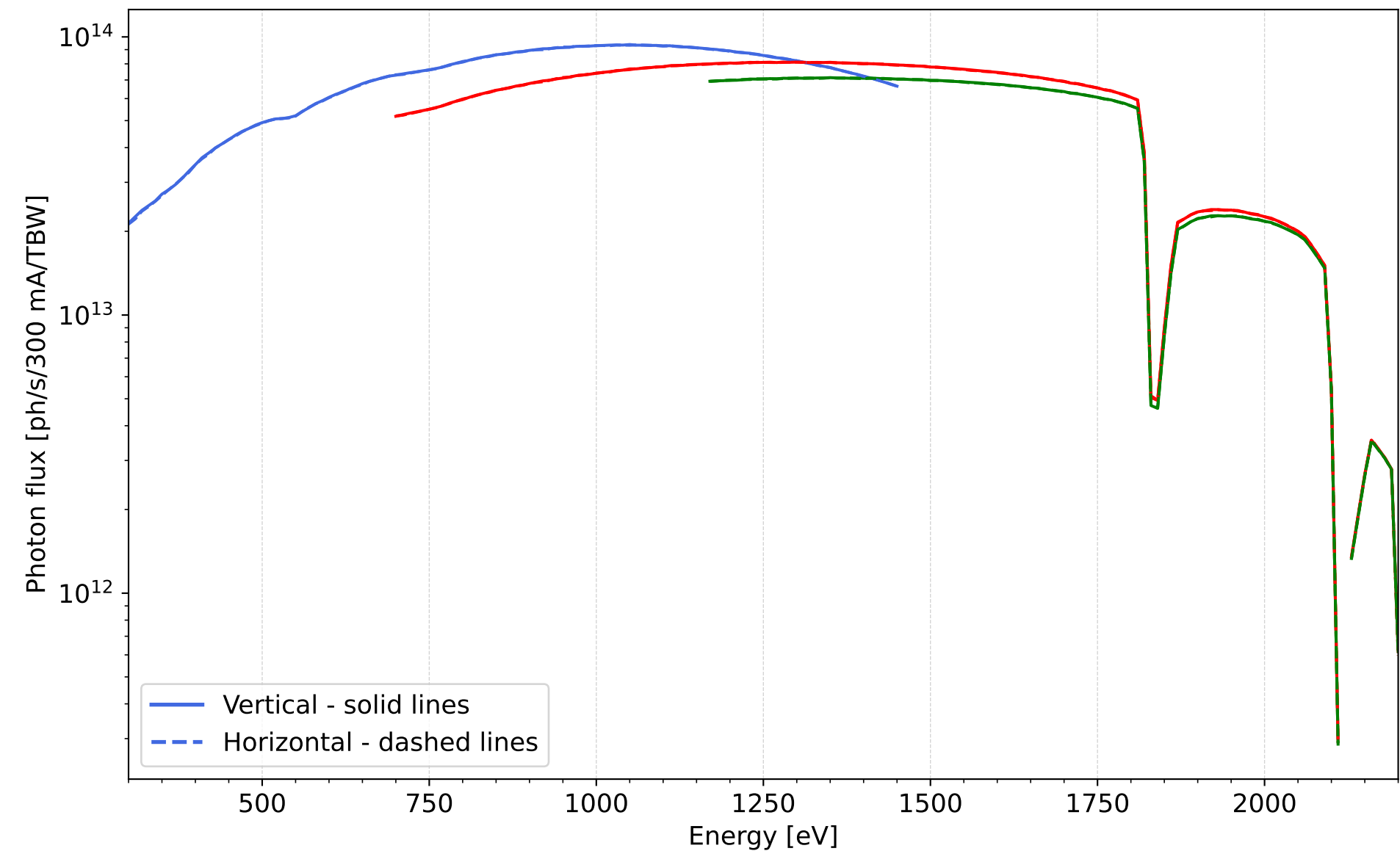
Flux at Focus
