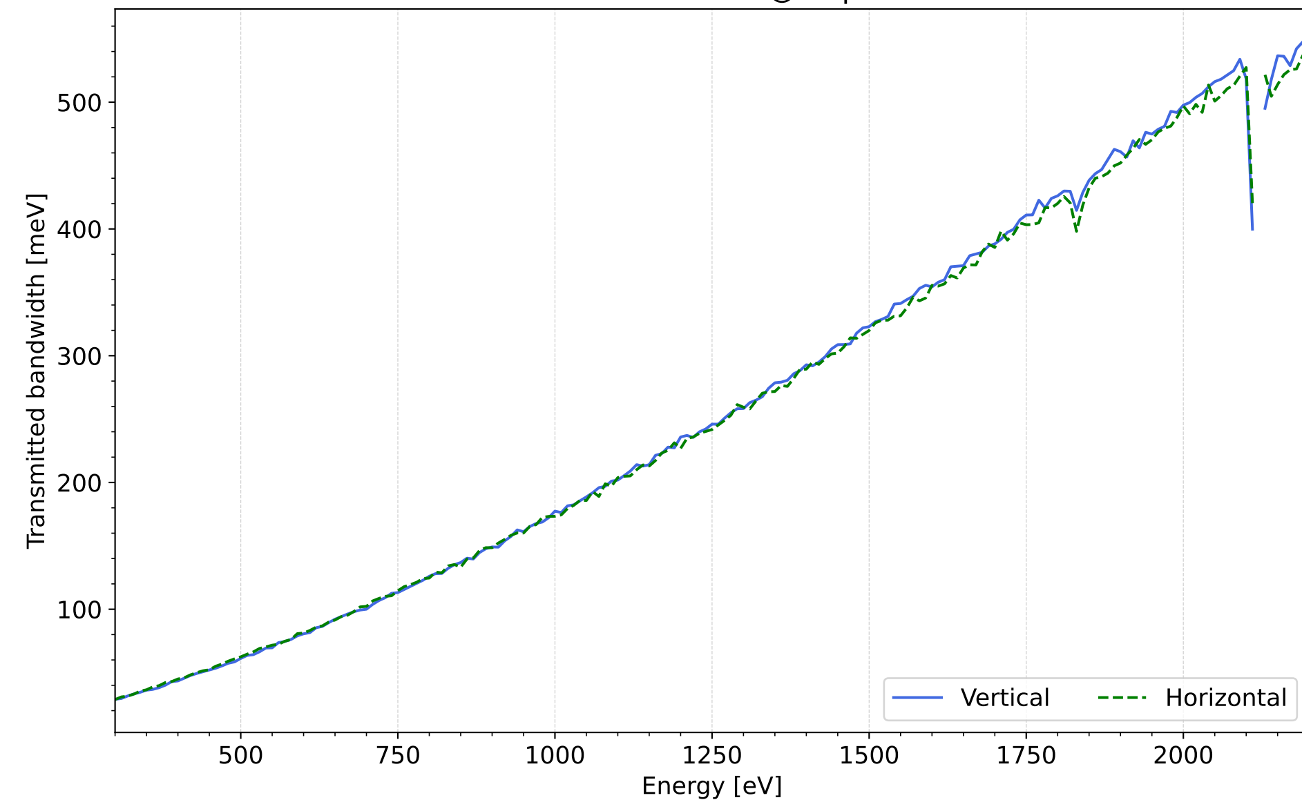
Transmitted Bandwidth @30 \mu\text{m} ExitSlit
