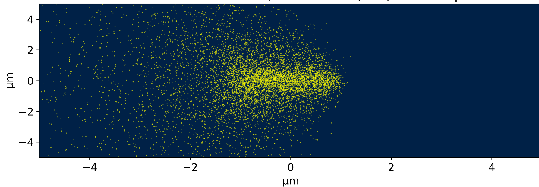
Horizontal Monochromator, Focus FWHM(HxV) 2.0 x 1.5 \mu\text{m}^2
