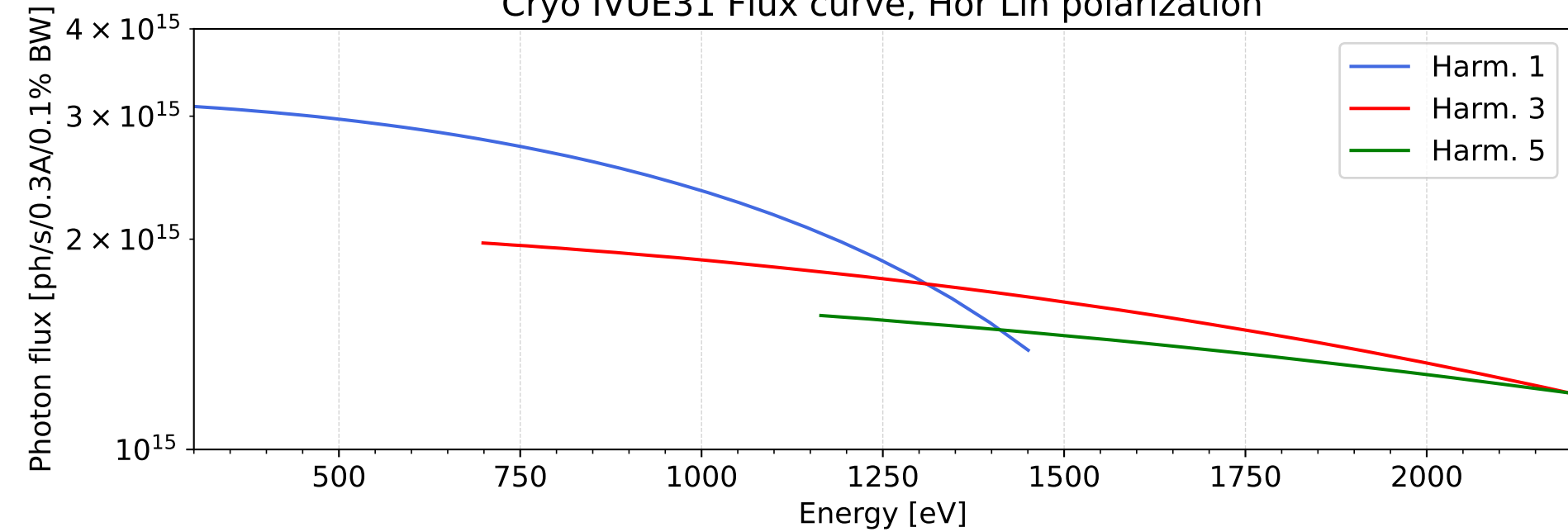
Flux at Focus
