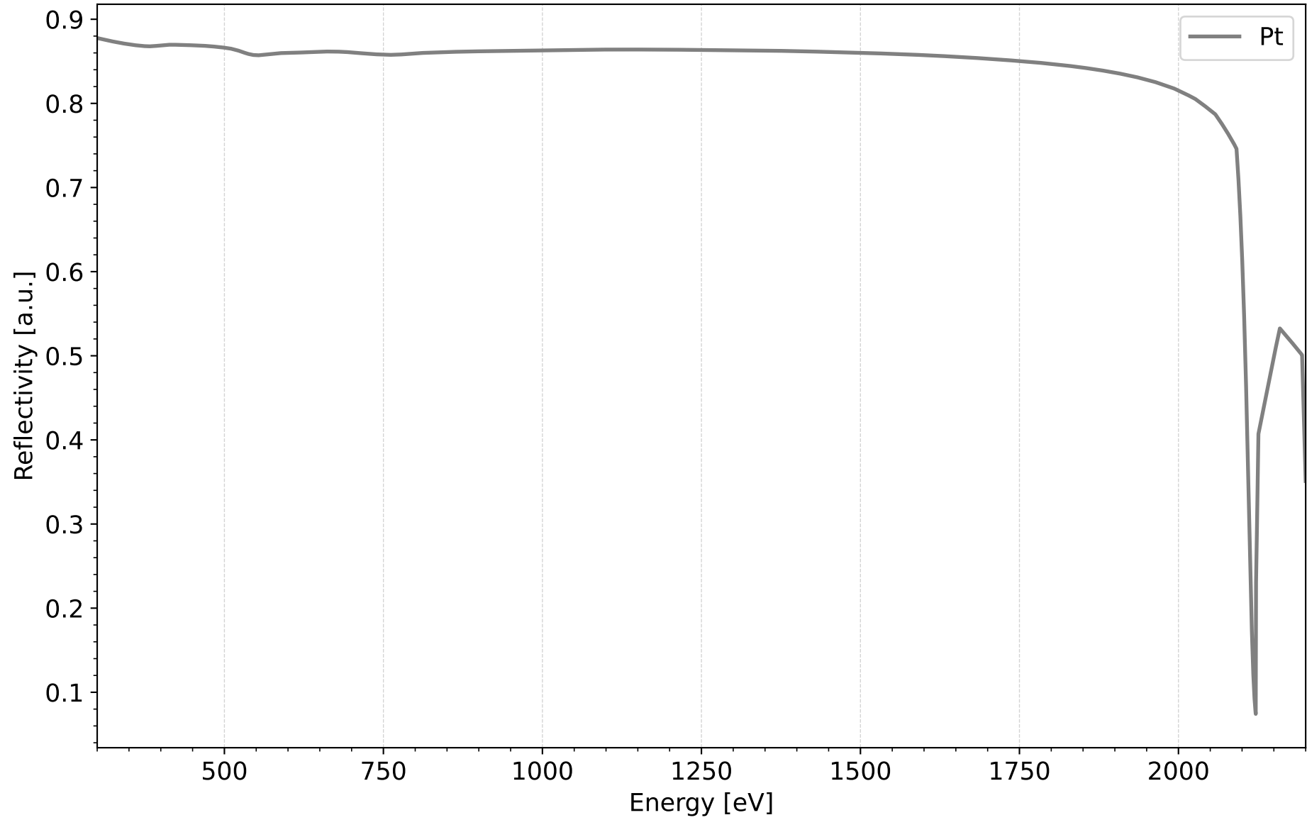
Mirror Coating Reflectivity @ 0.7° incident angle
