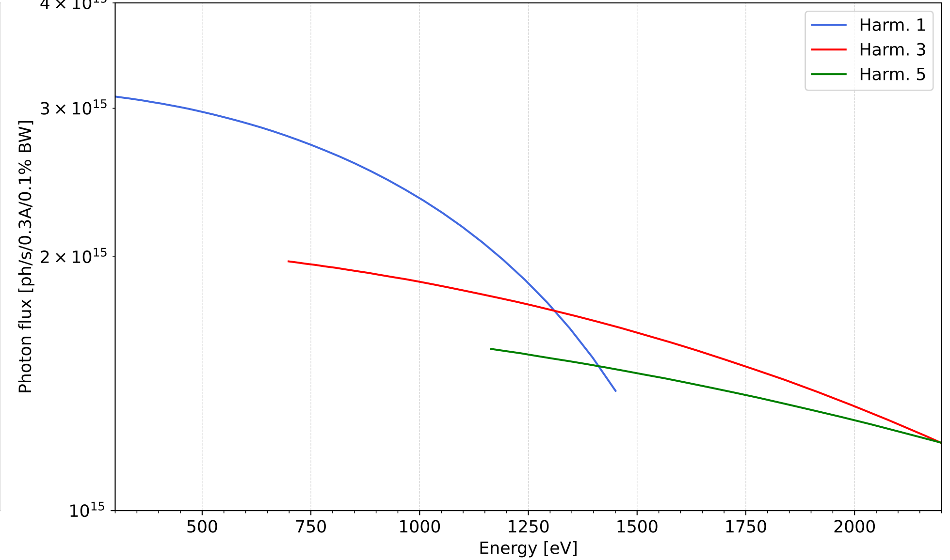
Cryo IVUE31 Flux curve, Hor Lin polarization
