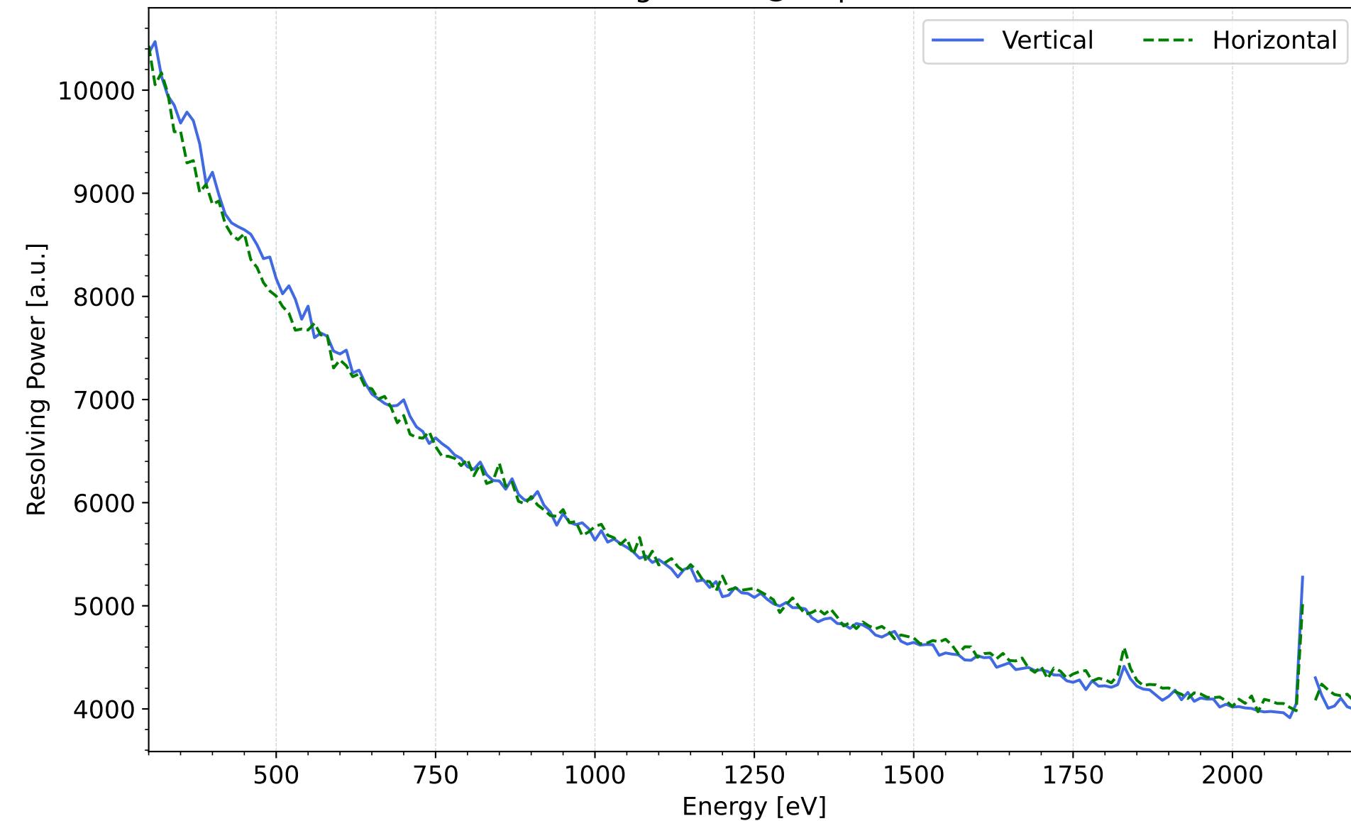
Resolving Power @30 \mu\text{m} ExitSlit
