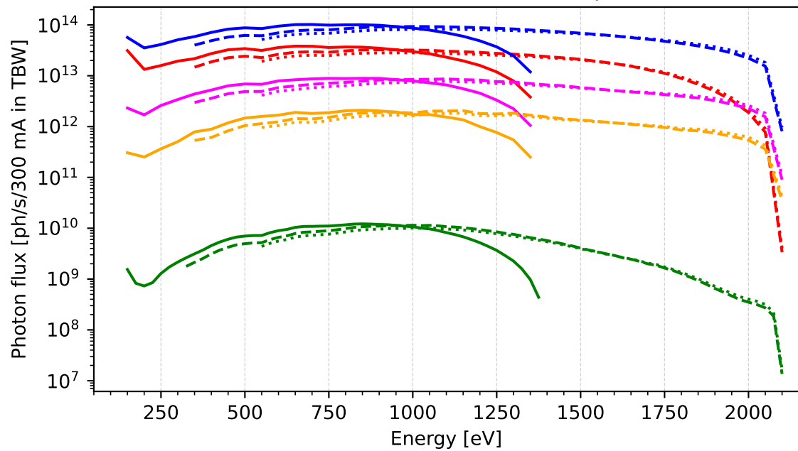
Flux Density on sample
