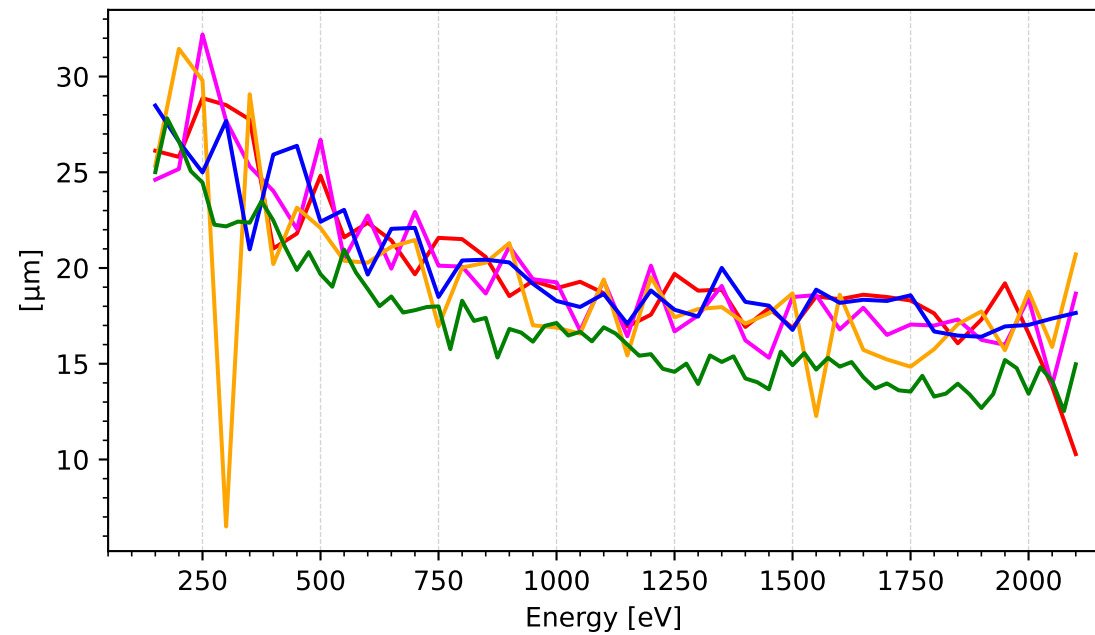
Horizontal Focus Size
