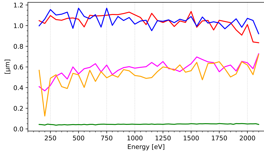
Vertical Focus Size
