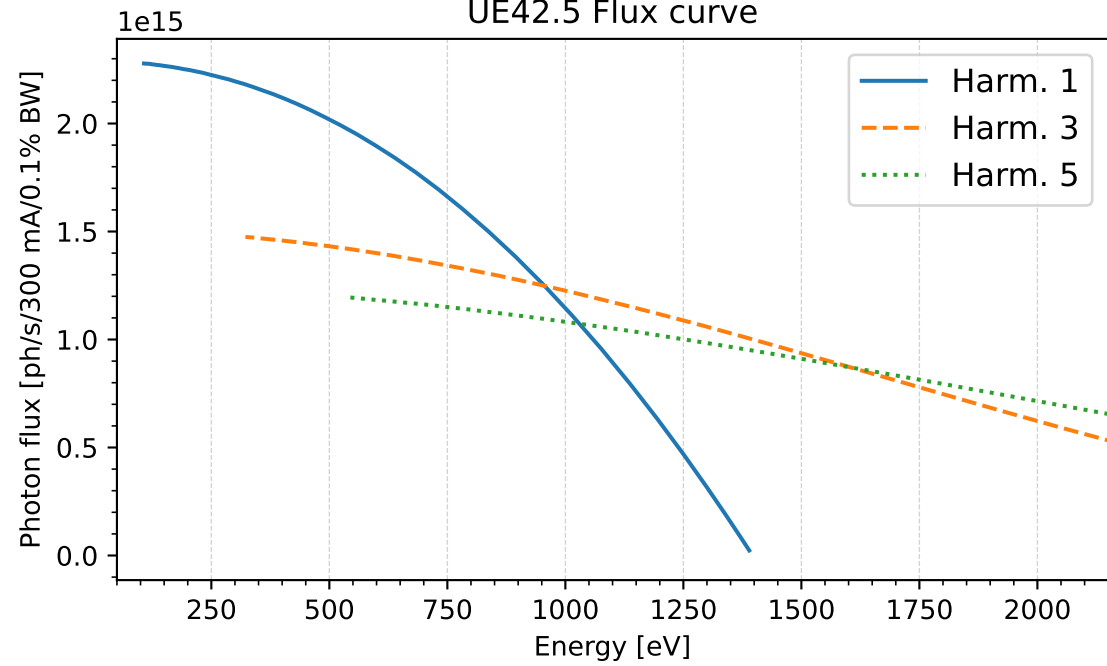
Transmitted flux (Flux on sample)
