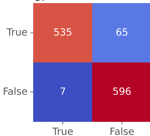
gpt-4o-mini with MV
