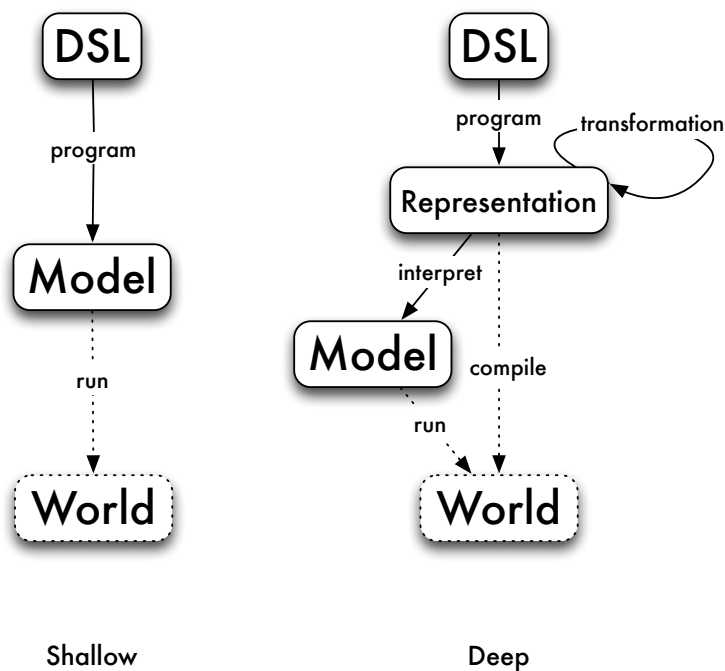
Figure 20.3: Shallow and deep embeddings
