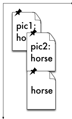
Figure 20.4: Positioned images
