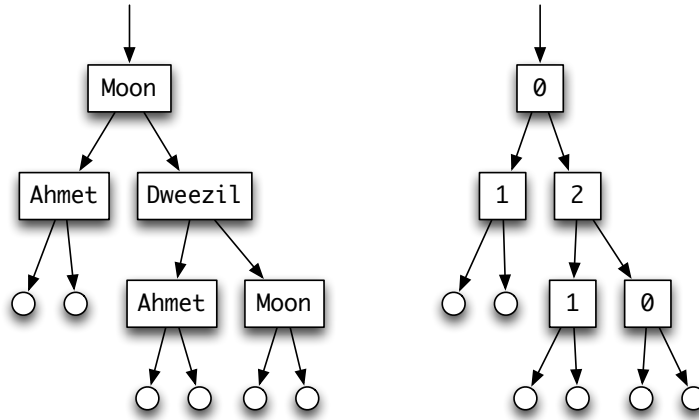
Figure 19.1: Replacing the elements of a tree with natural numbers.
