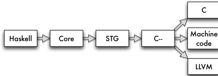
Figure 20.1: Languages in the Glasgow Haskell Compiler
