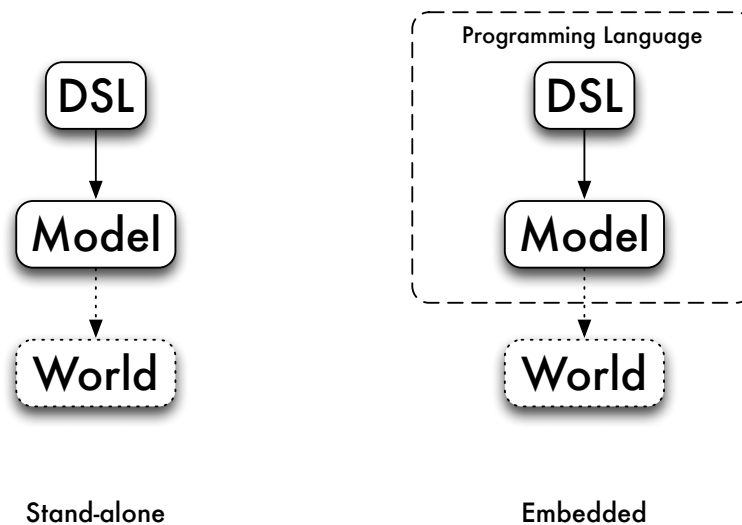
Figure 20.2: Stand-alone and embedded DSLs
