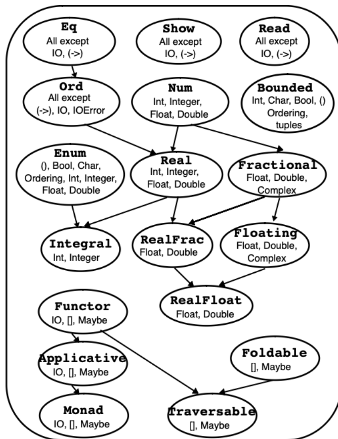
Figure 13.1: The Haskell Base classes 2
