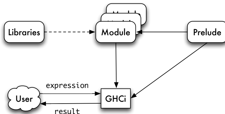
Figure 2.5: GHCi, Prelude and other modules
