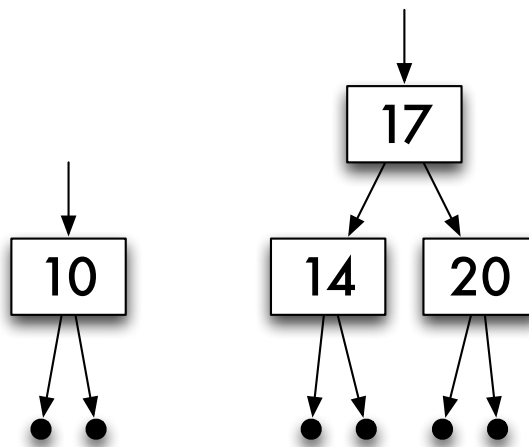
Figure 14.2: Two trees.
