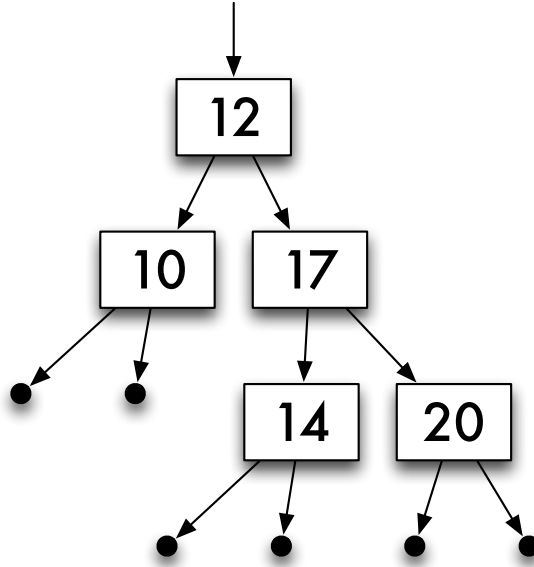
Figure 14.1: An example of a tree of integers.
