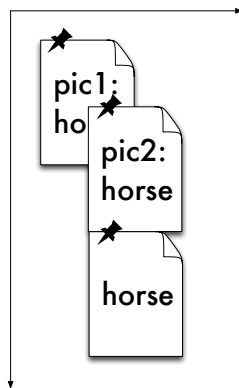
Figure 19.4: Positioned images
