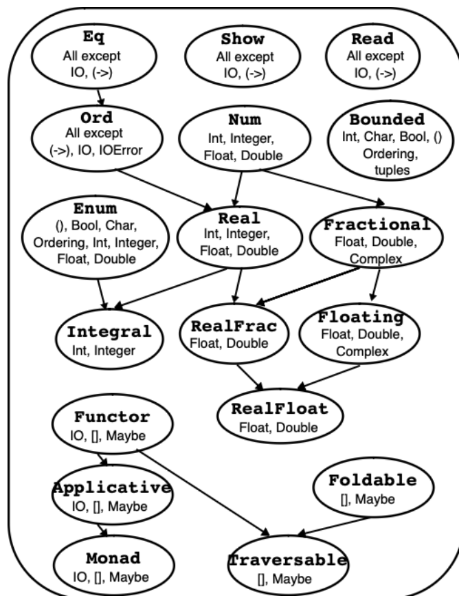
Figure 13.1: The Haskell standard classes 2
