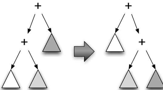
Figure 14.3: Rearranging additions
