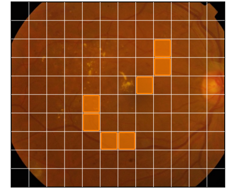
schematic selected witnesses M^*[k]
