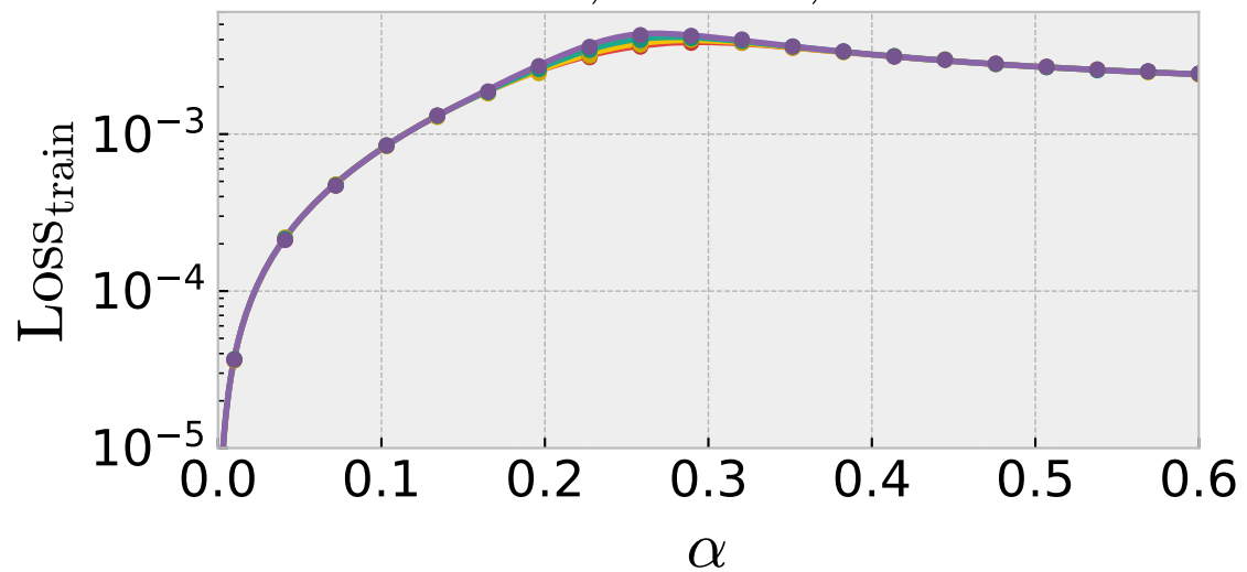
\lambda = 0.05, \kappa^* = 0.3, \Delta = 0.
