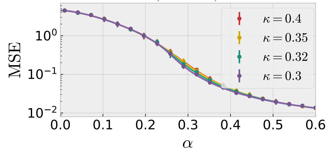
\lambda = 0.05, \kappa^* = 0.3, \Delta = 0.
