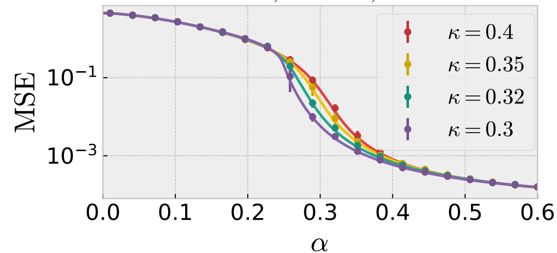
\lambda = 0.01, \kappa^* = 0.3, \Delta = 0.
