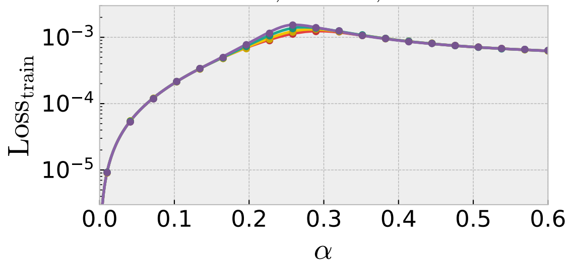
\lambda = 0.01, \kappa^* = 0.3, \Delta = 0.
