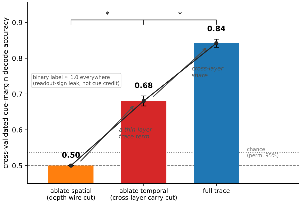
Lower-layer cue credit: a ladder across the two trace terms
