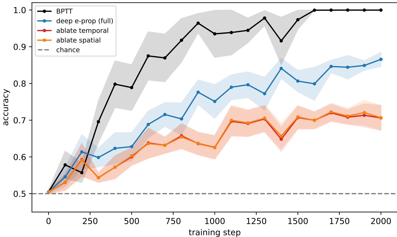
Exp 5.2 — BPTT \geq full e-prop > controls (D=12, n=8 seeds, \pm SEM)
