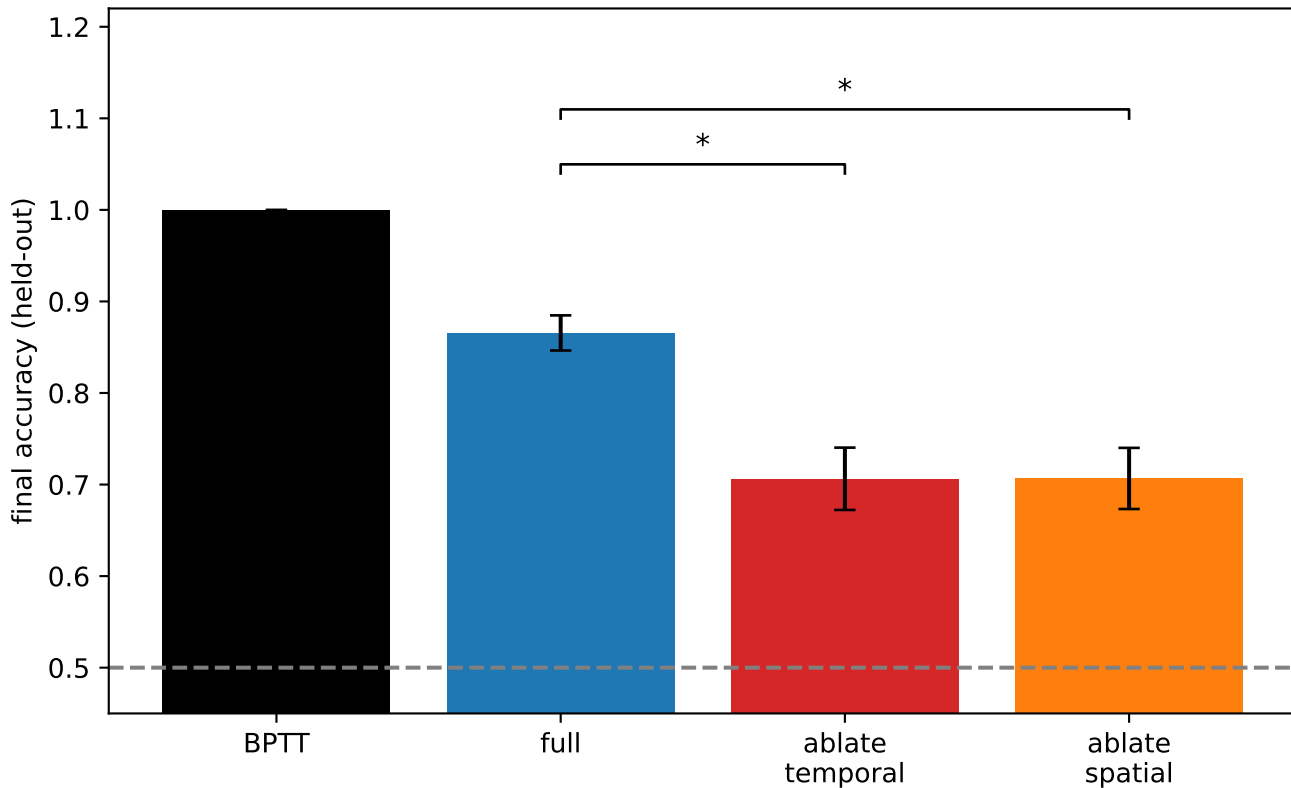
Exp 5.3 - final accuracy with significance (n=8 seeds, +/-SEM) brackets: full vs control, Holm-corrected sign-flip permutation
