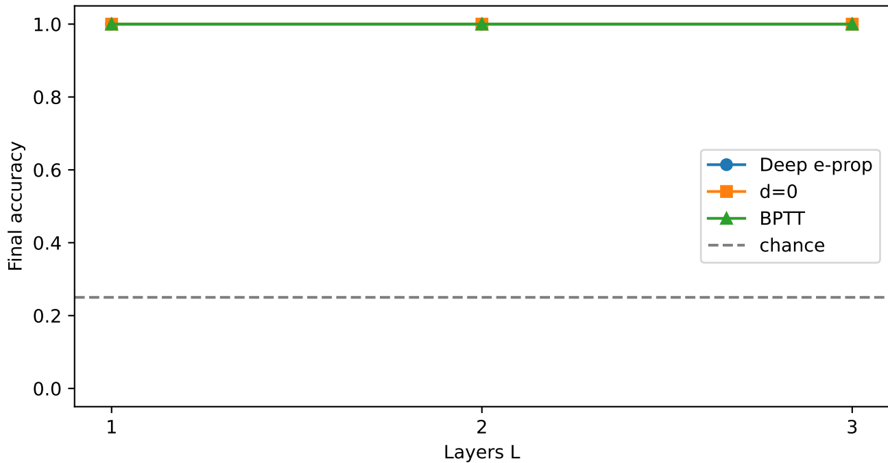
Final accuracy vs depth — store-and-recall (delay=2)
