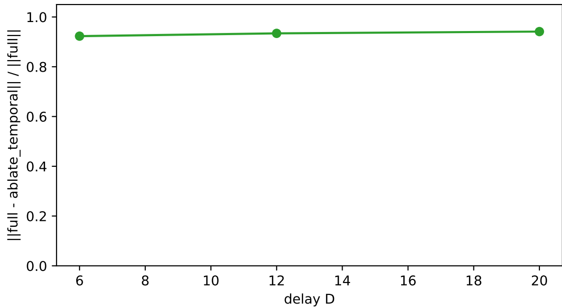
Lower-layer credit via cross-layer trace \epsilon^z
