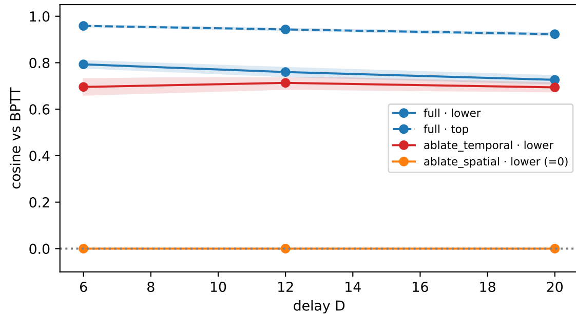
Per-layer credit alignment
