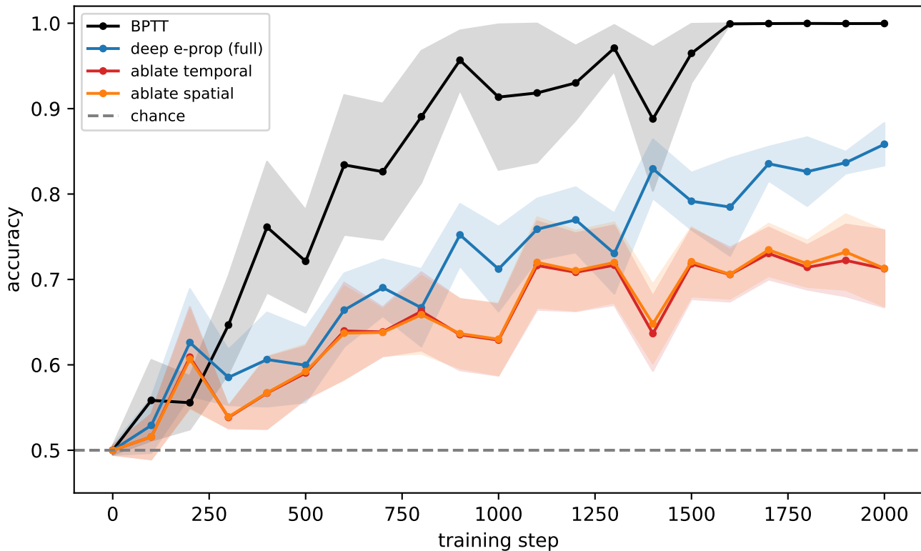
Exp 5.2 — BPTT \geq full e-prop > controls (D=12, n=6 seeds, \pm SEM)
